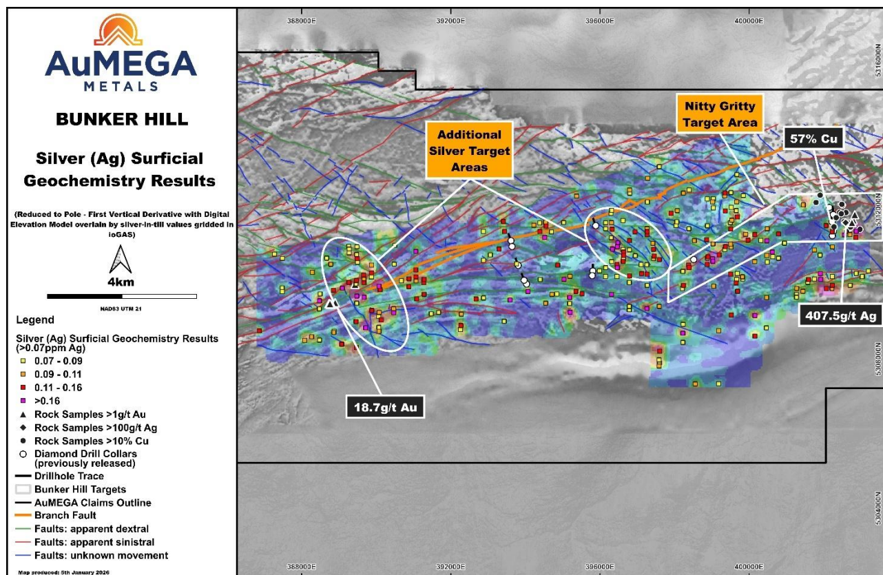
Figure 7: Silver-in-till results from Bunker Hill. The figure contains gridded silver-in-till overlying the greyscale reduced to pole – fist vertical derivative magnetics. Results are filtered to >0.07ppm silver.
