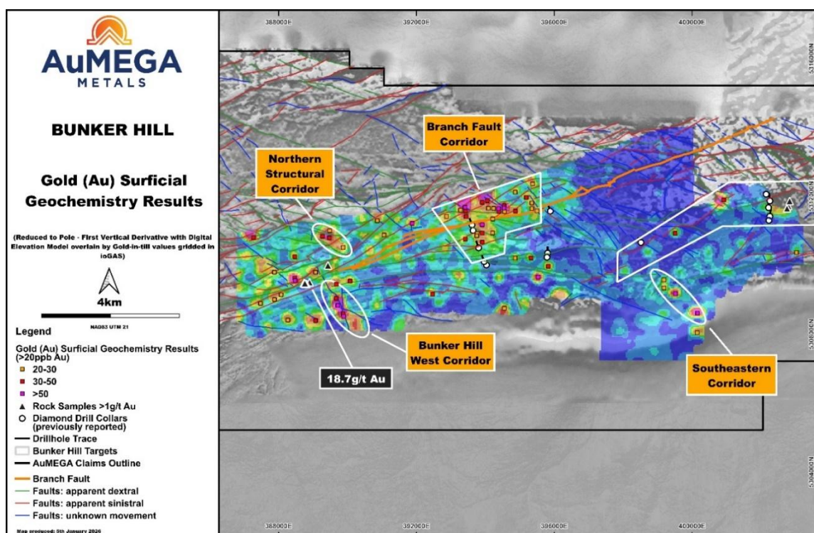
Figure 3: Gold-in-till results from Bunker Hill. The figure shows gridded gold-in-till results overlying the greyscale reduced to pole – first vertical derivative magnetics. The gold-in-till results are filtered to >20 ppb gold.
