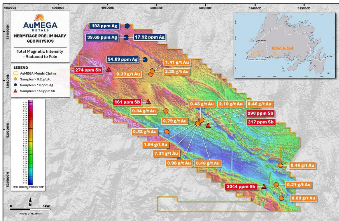
Figure 9: Hermitage high-resolution airborne magnetic survey and rock sample results.
