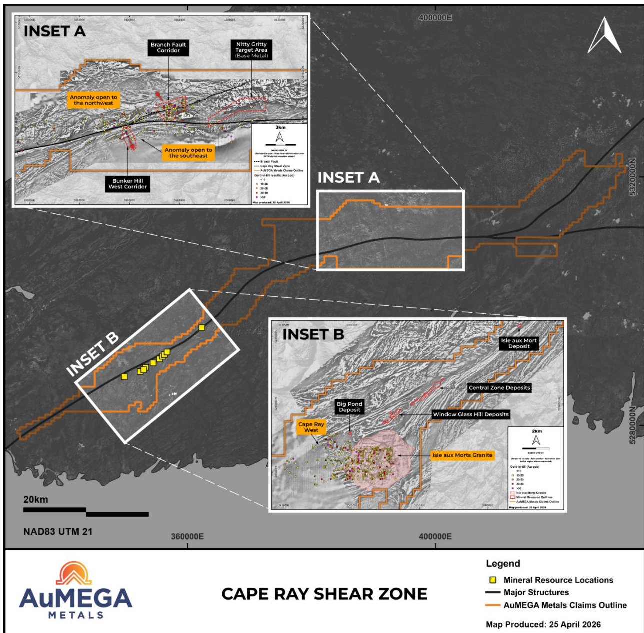
Figure 2. Surficial geochemistry overview for 2026.
