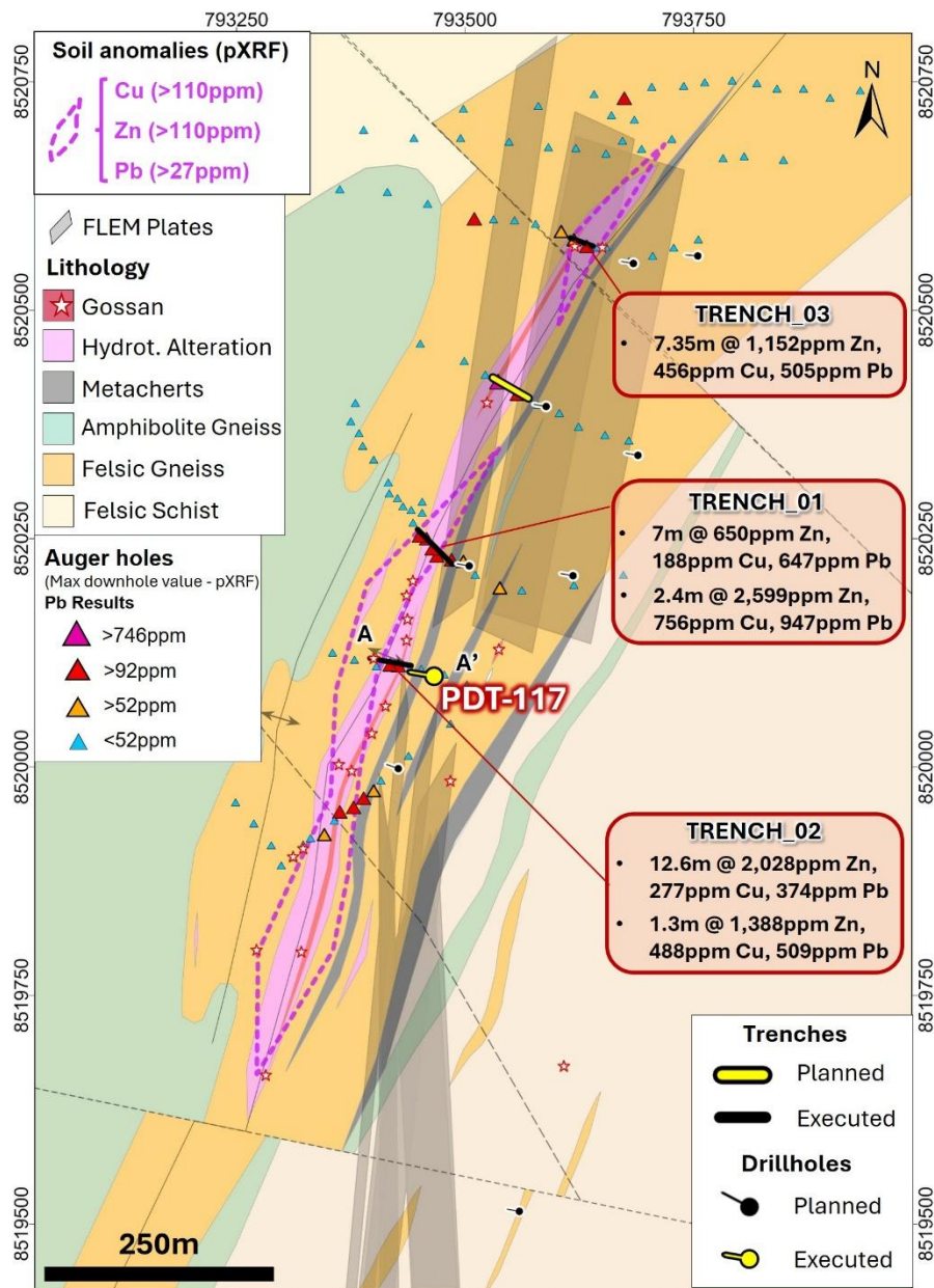
Figure 2: Touro Prospect plan, first hole of the current campaign- PDT_117 which intersected massive sulphide mineralisation. Trench locations, geochemical anomaly, gossans and the hydrothermal alteration zone.
