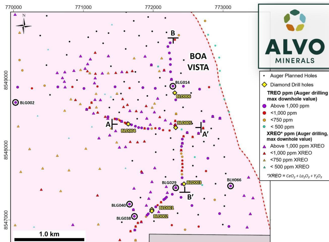
Figure 5: Bluebush IAC HREE Project, Boa Vista prospect plan showing diamond and auger drilling.
