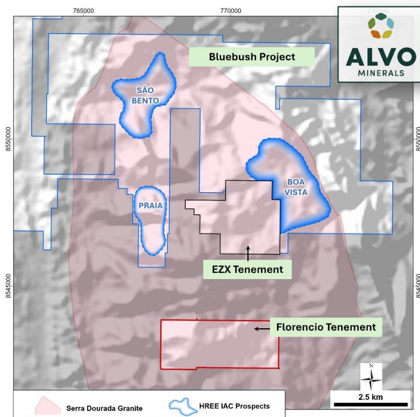
Figure 2: The Florencio tenement (red) relative to the Serra Dourada granite, the Bluebush and EZX tenements and the Serra Verde mining concessions.
