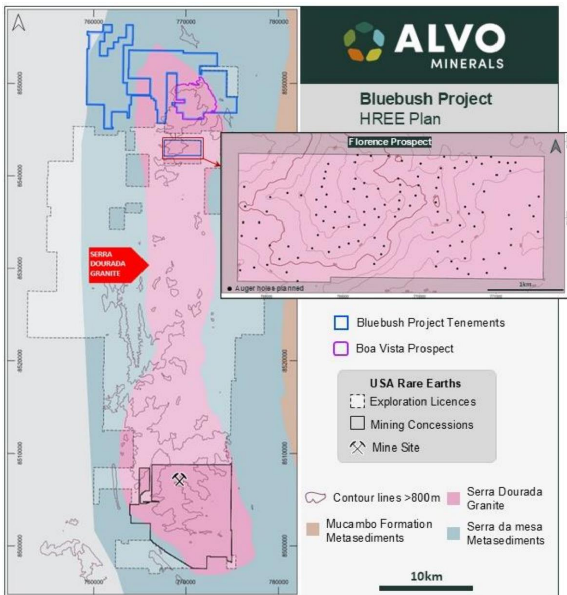
Figure 1: Regional map showing Bluebush on the northern end of the Serra Dourada granite, host to the Serra Verde (USA Rare Earth) ionic clay HREE operation (south end) in Central Brazil.
