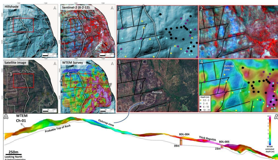
Figure 8: Boa Vista prospect. Upper panels: terrain hillshade, Sentinel 2 satellite composite, satellite image and EM survey response, with auger holes coloured by depth. Lower panel: section A to A' looking north (3x vertical exaggeration) with diamond holes BLD004 and BLD005.
