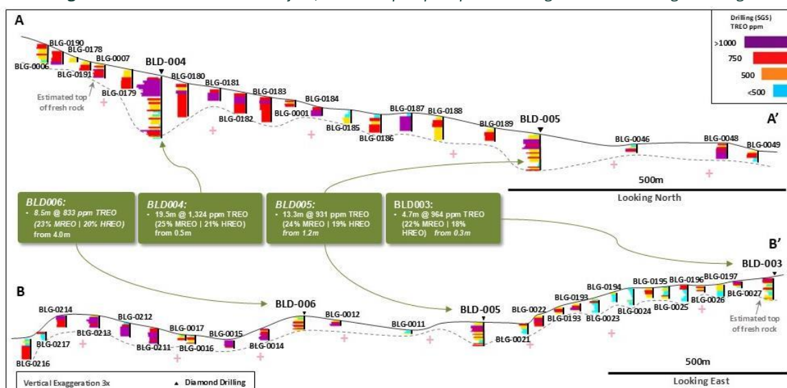
Figure 6: Cross sections through Boa Vista, Bluebush.
