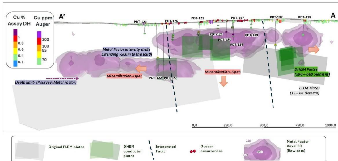
Figure 10: Touro prospect long section (looking west), including Metal Factor intensity shells (purple), FLEM (grey) and DHEM (green) survey results.
