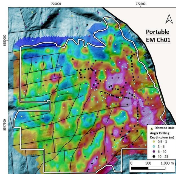
Figure 9: Boa Vista EM survey response (CH01) with auger holes labelled and coloured by depth (m). Stronger responses (red to pink) coincide with deeper drill holes.
