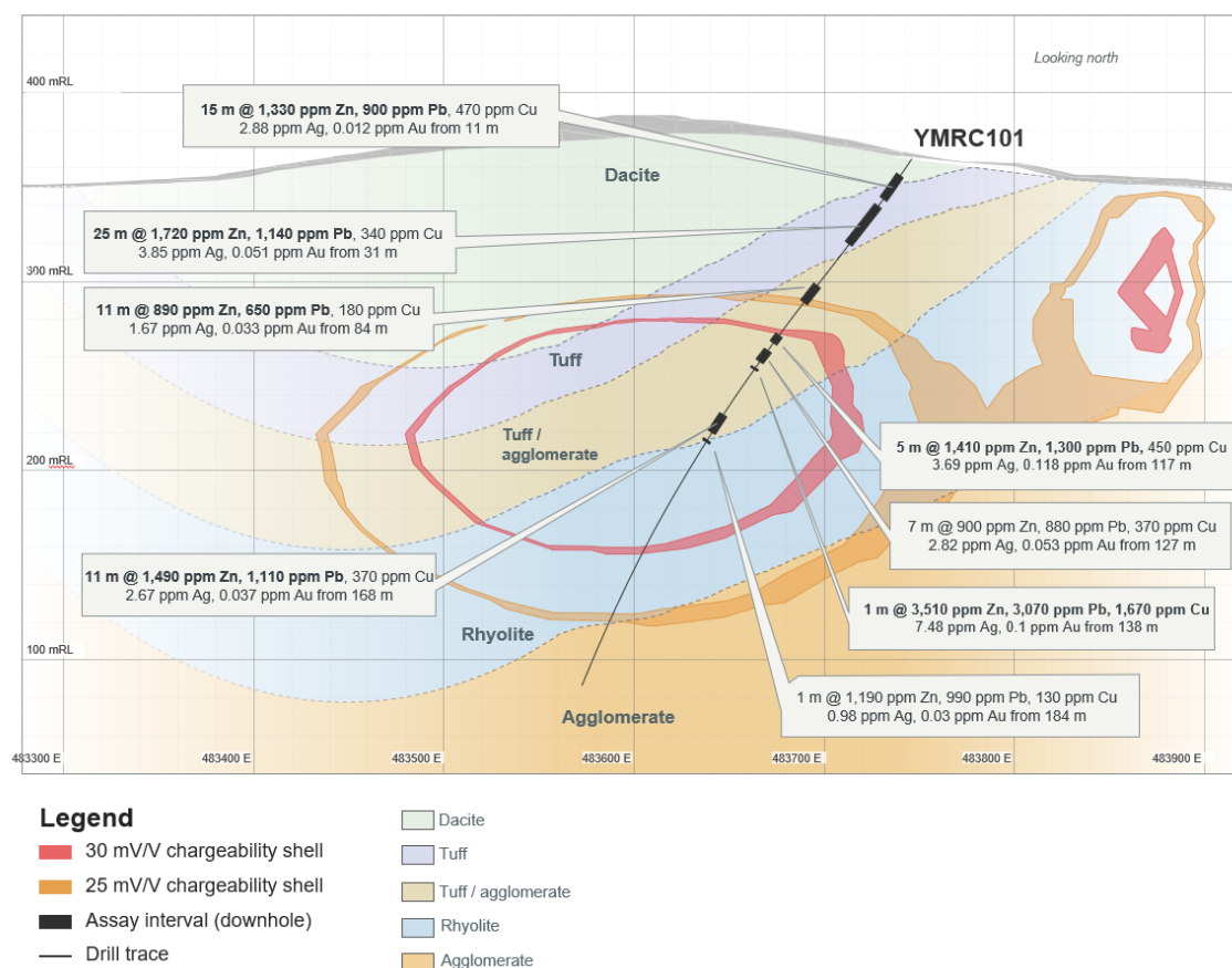
Figure 5: Yellow Mountain YMRC101 Cross Section
