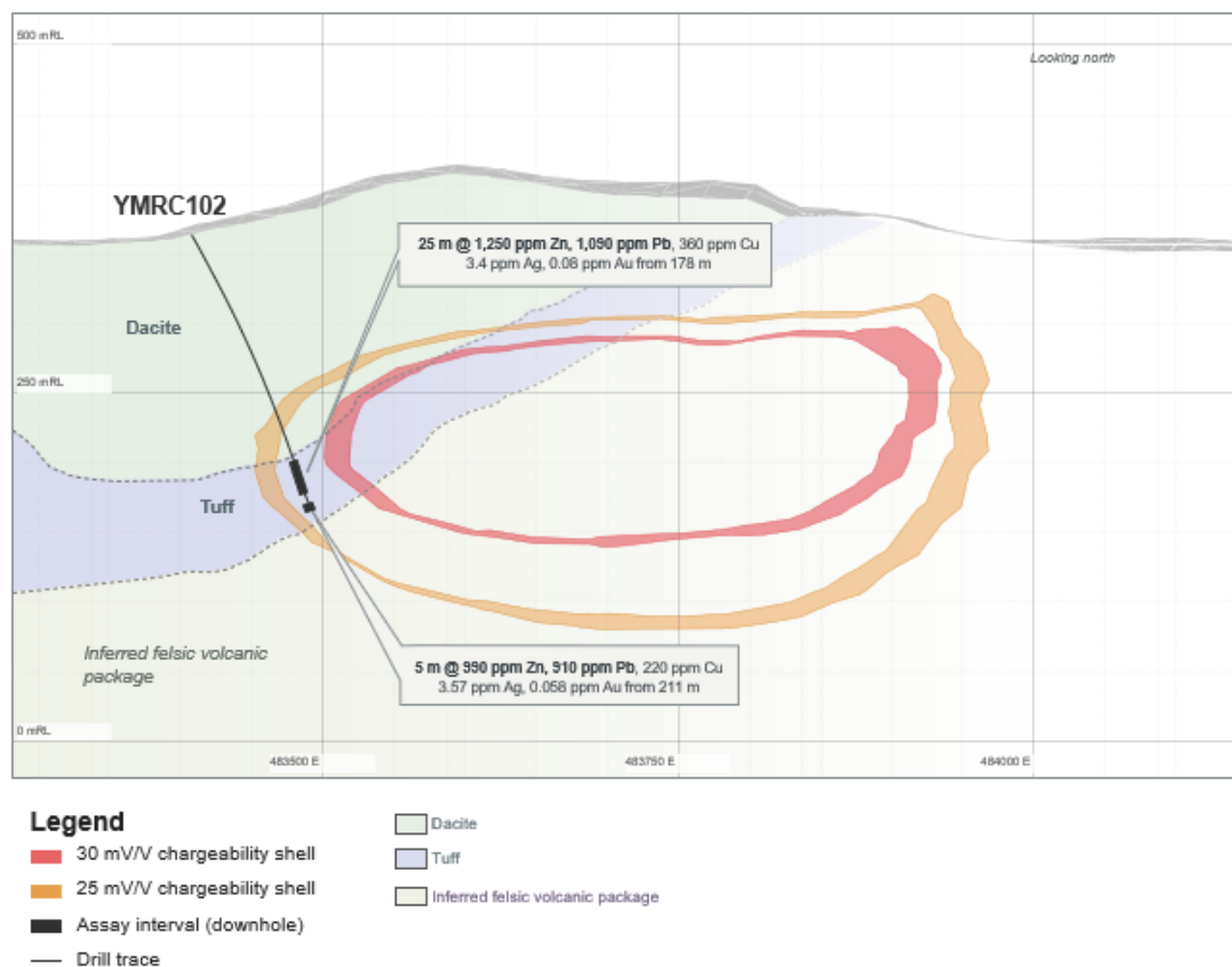
Figure 6: Yellow Mountain YMRC102 Cross Section
