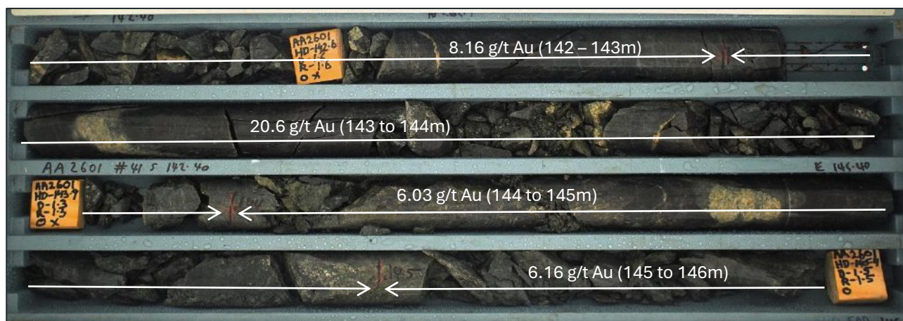
Figure 1: AA2601 – Tray #41 : 142.4m to 145.4m, gold assays annotated. Assayed grades only. No visual estimates of mineralisation.
