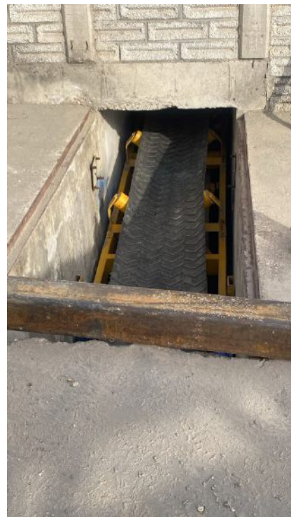
Figure 2: Conveyor to mill feed – belt refurbishment and installation of the mill feed conveyor
