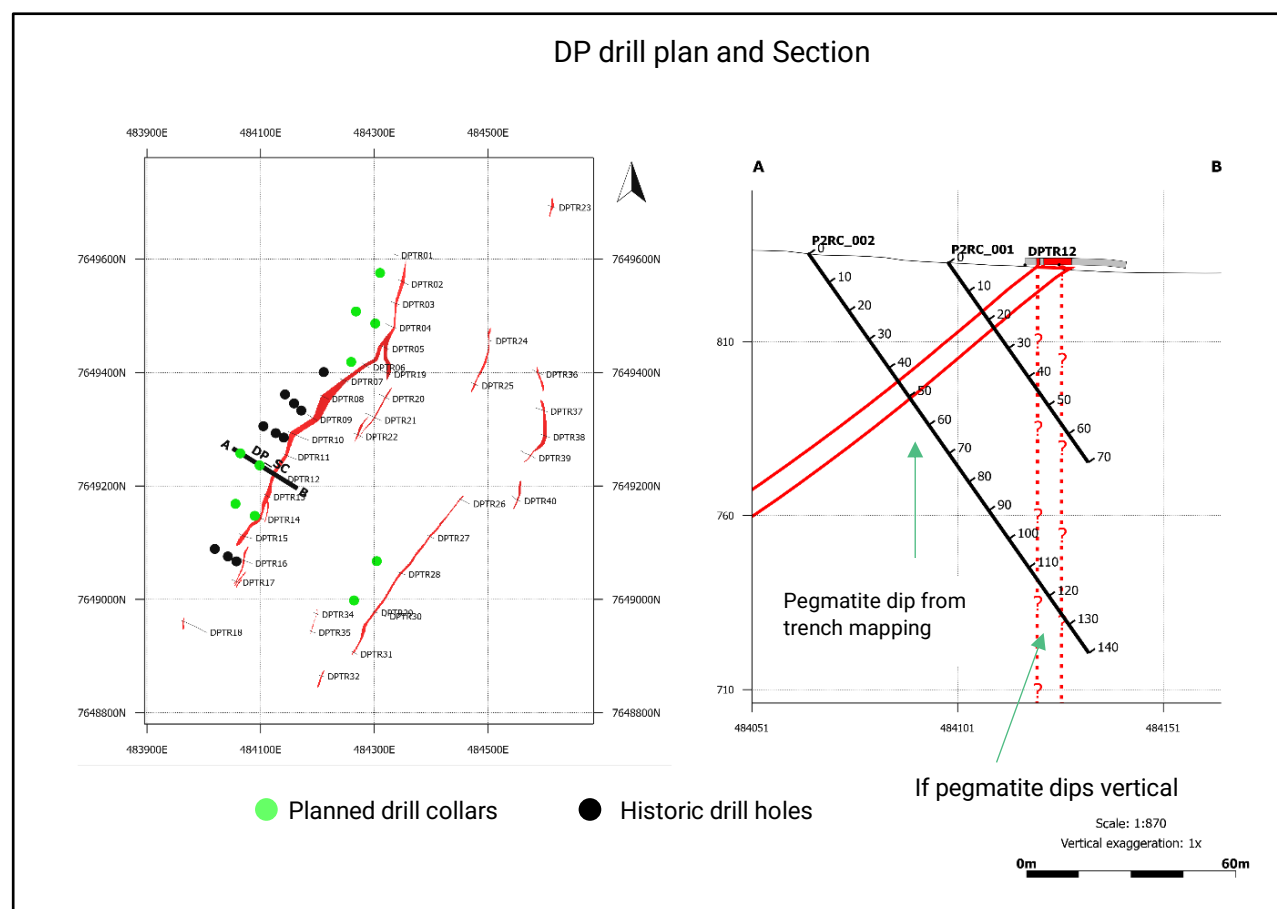
Figure 12: DP drill plan and section view
