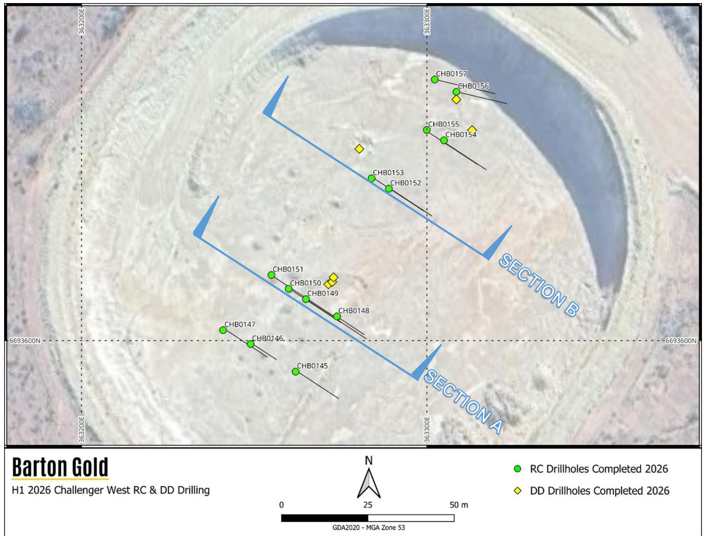
Figure 2 – Challenger West open pit plan map showing collar locations for new assays received
