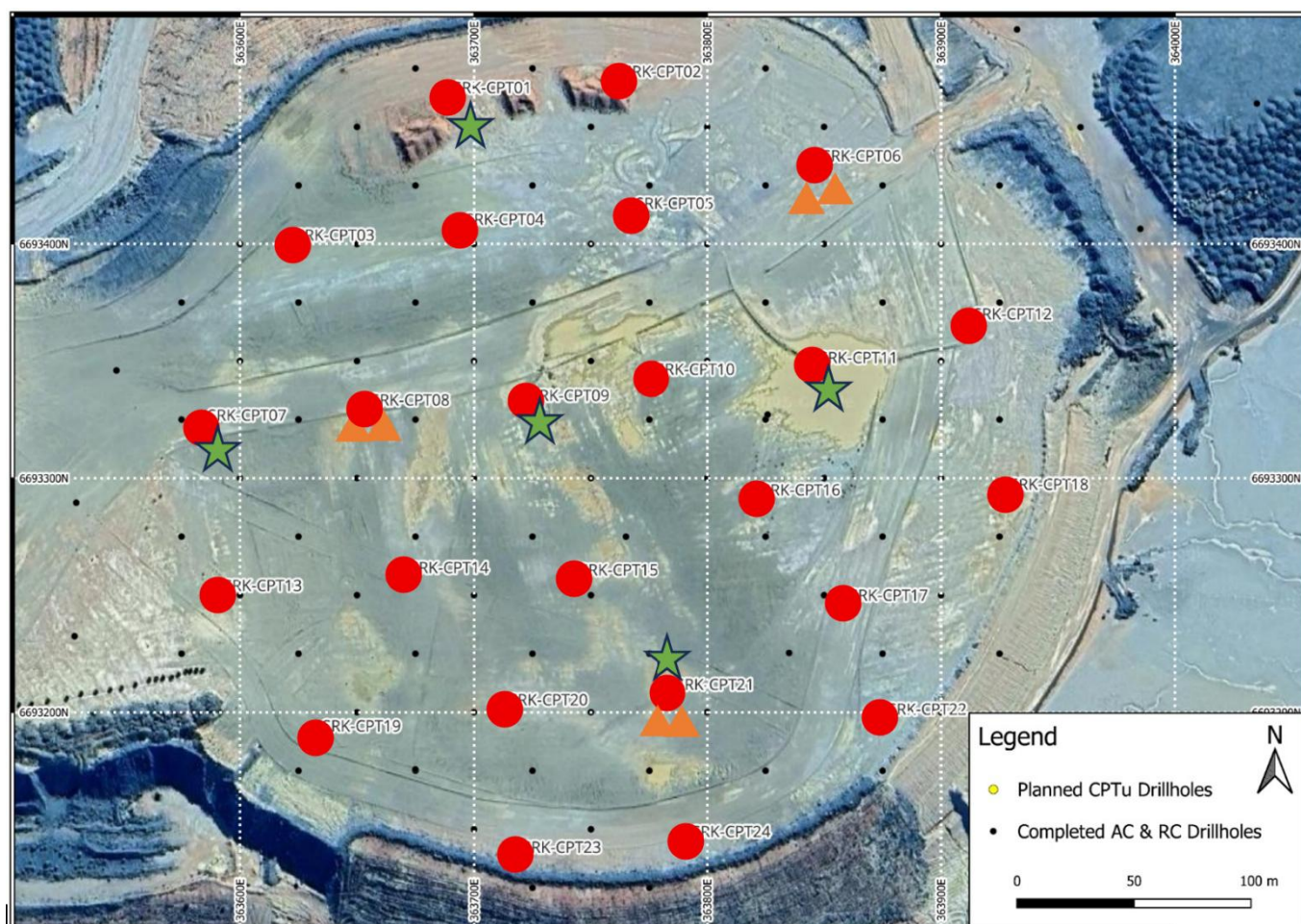
Figure 1 – TSF1 with completed CPT (red), sonic (green stars), VST / BD (orange) & AC / RC drill holes
