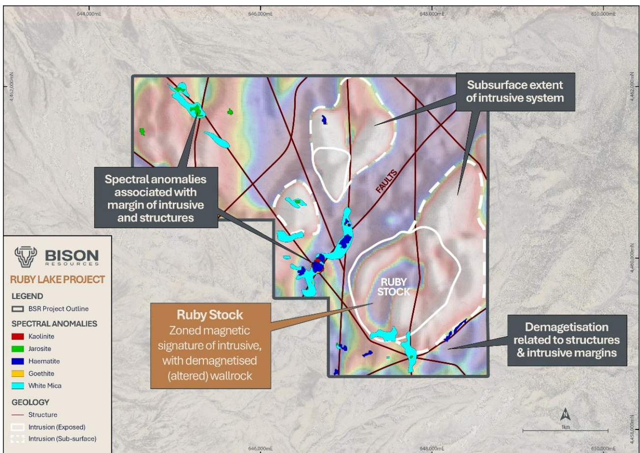
Figure 7: Ruby Lake Project – Spectral anomalies in relation to the surface expression of the Ruby Stock (solid white outline) relative to the sub-surface igneous complex (white dash outline) and structures (red lines). Underlain by TMI 1VD imagery 9 .
