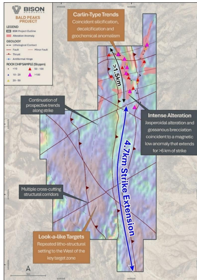
Figure 6: Bald Peaks Project – NNW-trending thrusts (thick red lines with teeth) and brittle faults (thin red lines) in relation to the surface geochemical anomaly, underlain by RTP tilt SE shade derivative imagery. Note the presence of the magnetic low anomaly coincident with surface geochemical anomalism that extends the full length of the Project 8 .
