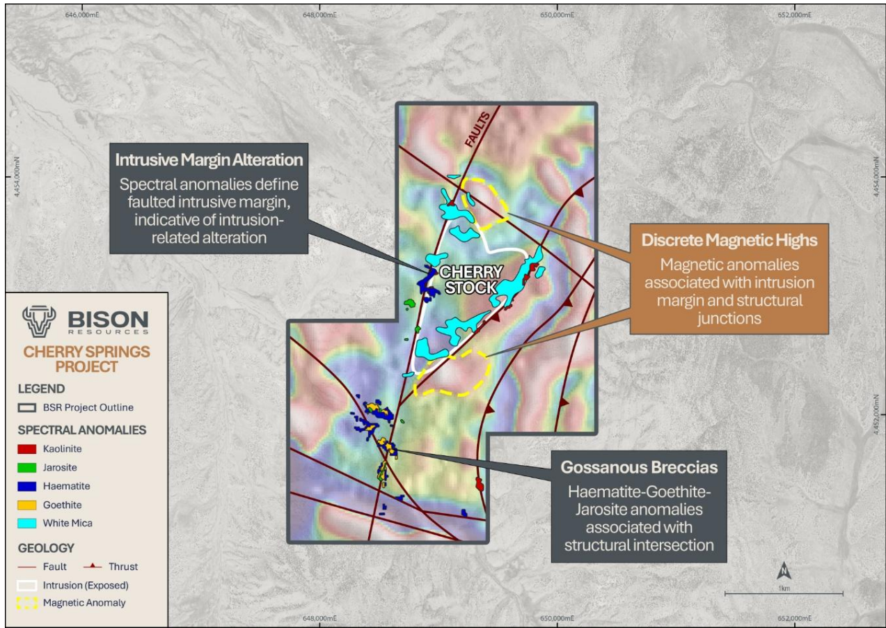
Figure 8: Spectral anomalies in relation to the surface expression of the Cherry Stock (solid white outline) relative to the discrete magnetic target anomalies (yellow dash outline) and structures (red lines). Underlain by TMI 1VD imagery 10 .
