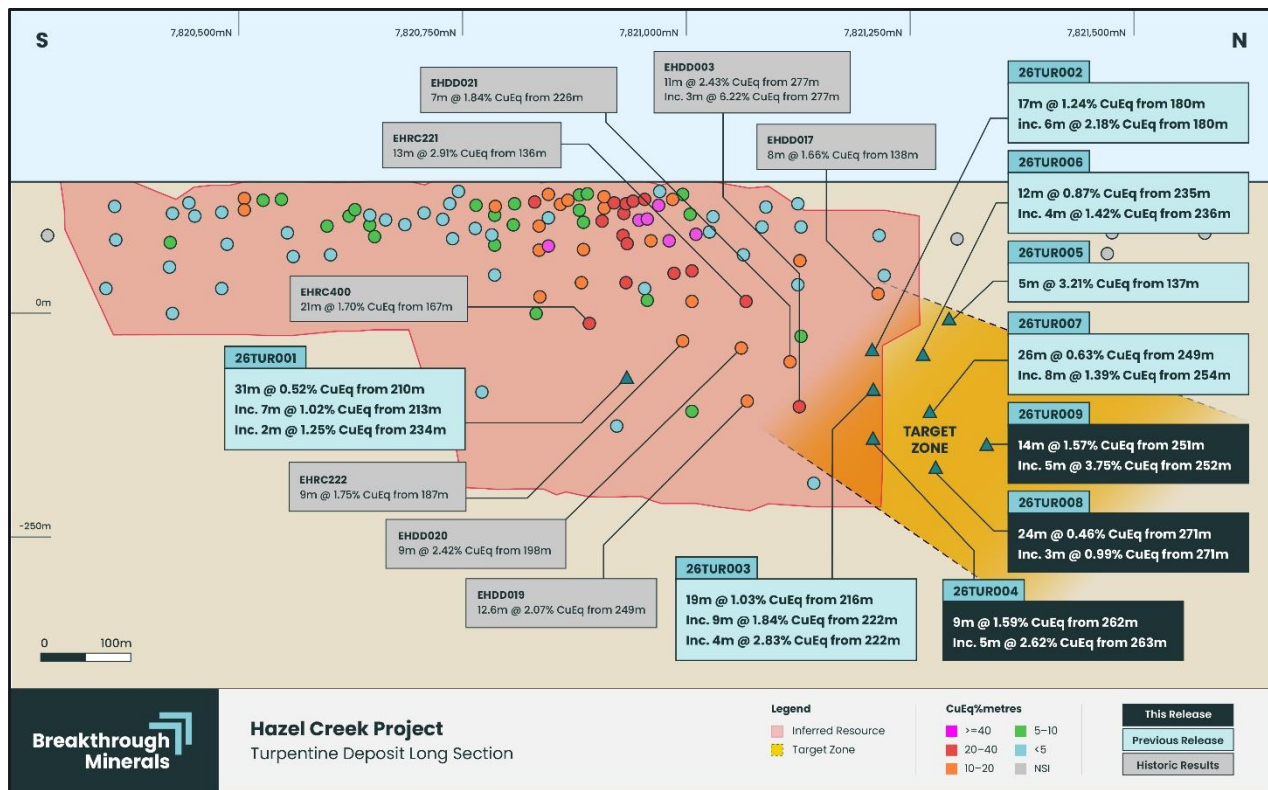
Figure 2: Turpentine long section showing the existing Mineral Resource model (red) and the position of 26TUR001–009 relative to the interpreted down-plunge extension
