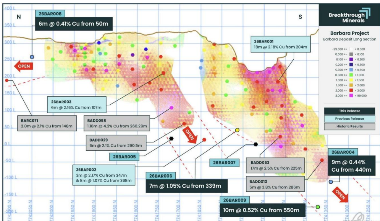
Figure 3: Barbara long section showing the existing Mineral Resource model and the position of 26BAR004, 26BAR006, 26BAR008 and 26BAR009
