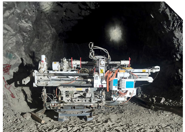
Figure 14 | Underground diamond drilling rig at Sierra Atacama
