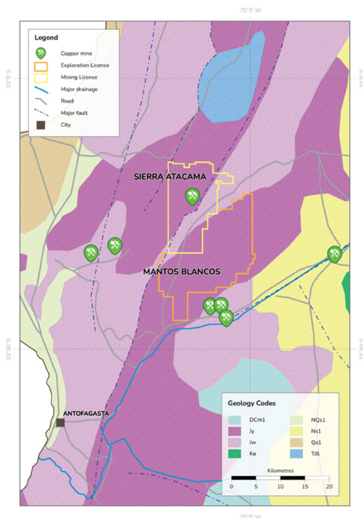
Figure 7 | Regional geological setting
