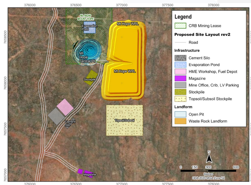
Figure 8 | Mount Hope Proposed Site Layout
