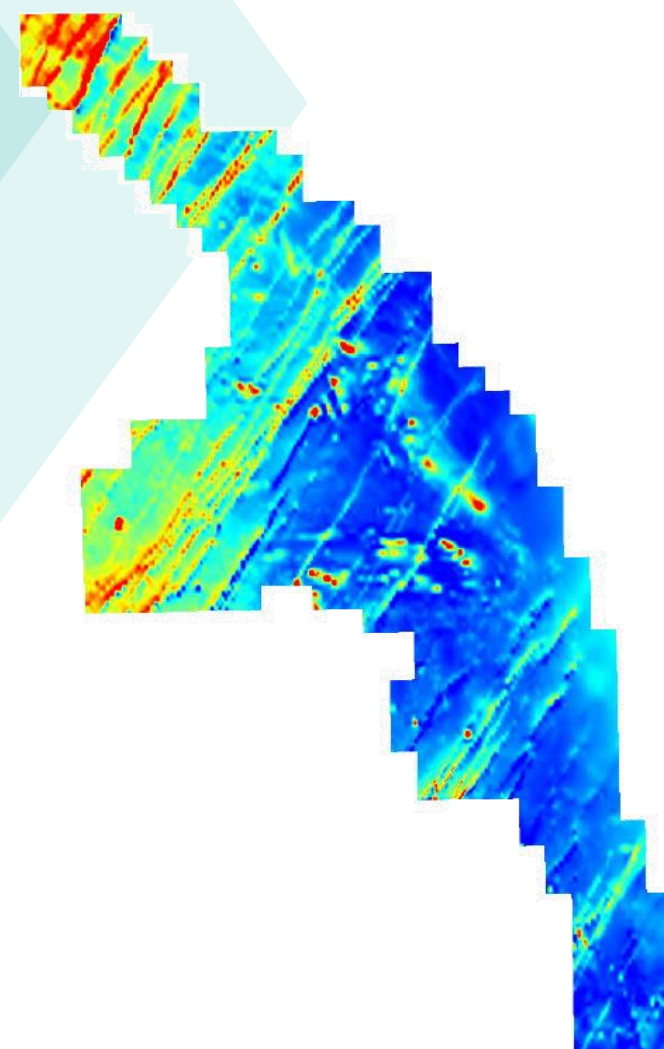
Magnetics Reduced to Pole (RTP)
