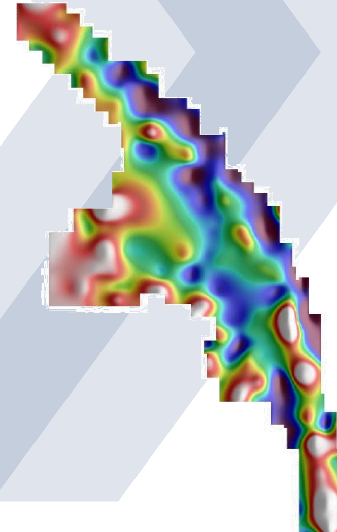
Regional Gravity
