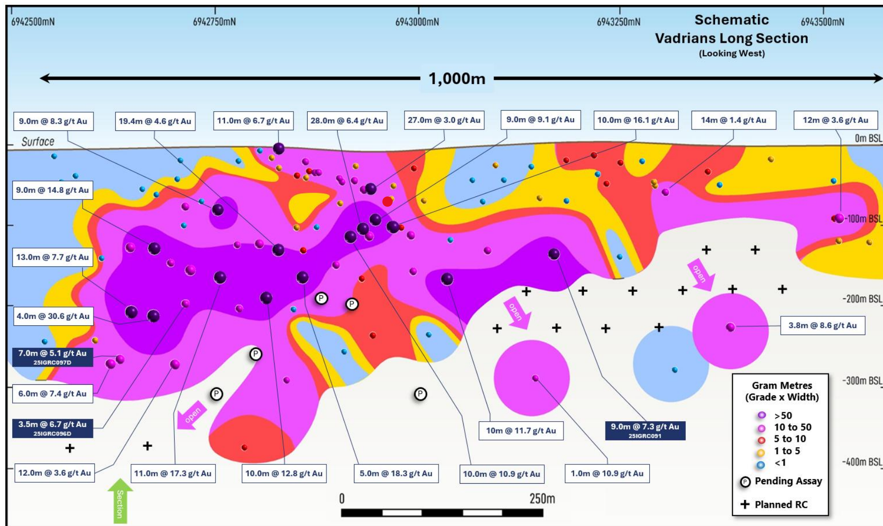
Figure 1: Schematic long section of the Vadrians gold deposit showing recent significant drill intersections (blue boxes) interpreted utilising ioGAS™.
