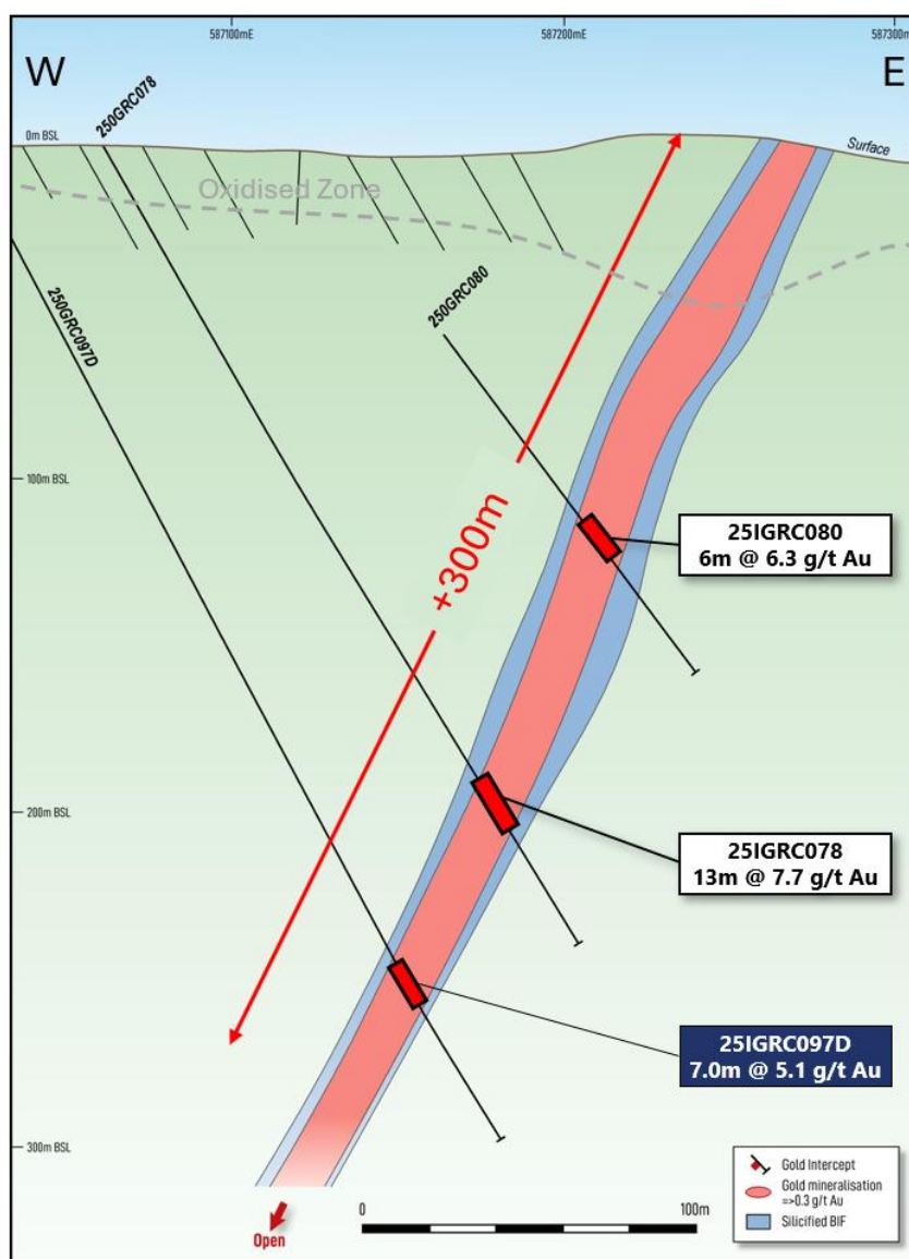
Figure 2: Schematic cross-section of the Vadrians gold deposit showing recent drill intersections (blue box).
