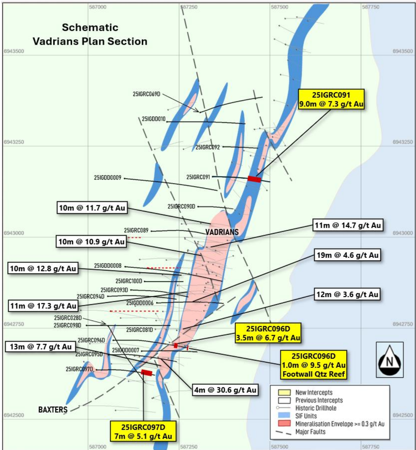
Figure 3: Schematic plan of Vadrians gold deposit highlighting recent significant drill results (yellow boxes).
