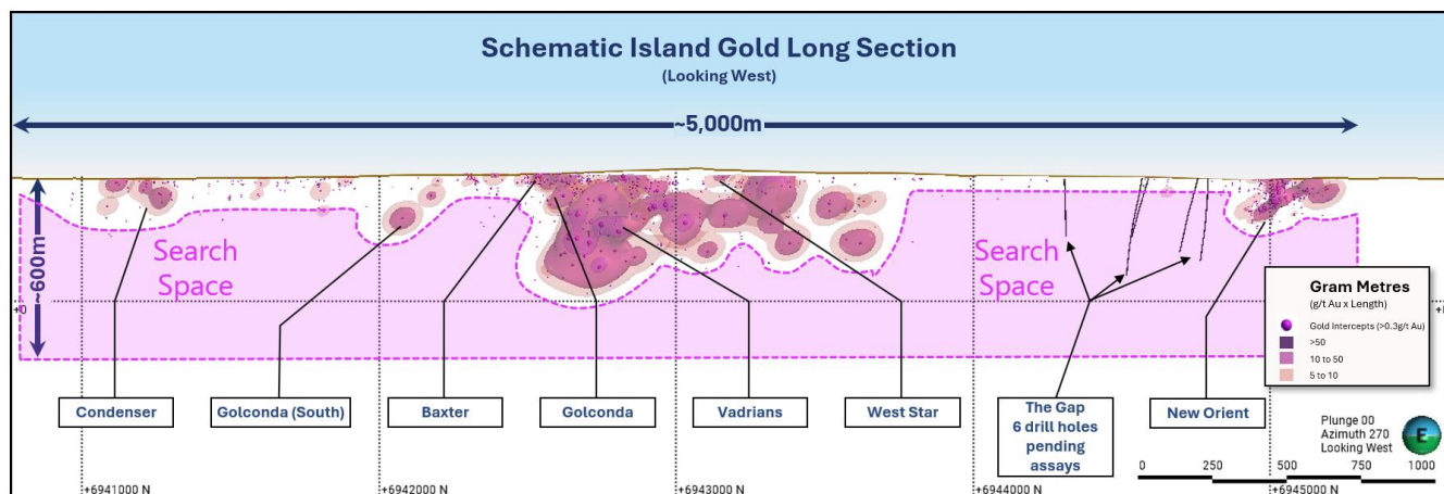
Figure 3: Schematic IGP Long Section showing gold mineralisation from Condenser in the south, Vadrians in the centre and New Orient in the north covering a strike length of +5km ; there are ten stacked BIF host rock units across the Island providing 50 strike-kilometres of highly prospective BIF , including high-grade gold mineralisation exceeding 400m vertical metres below the surface at Vadrians.
