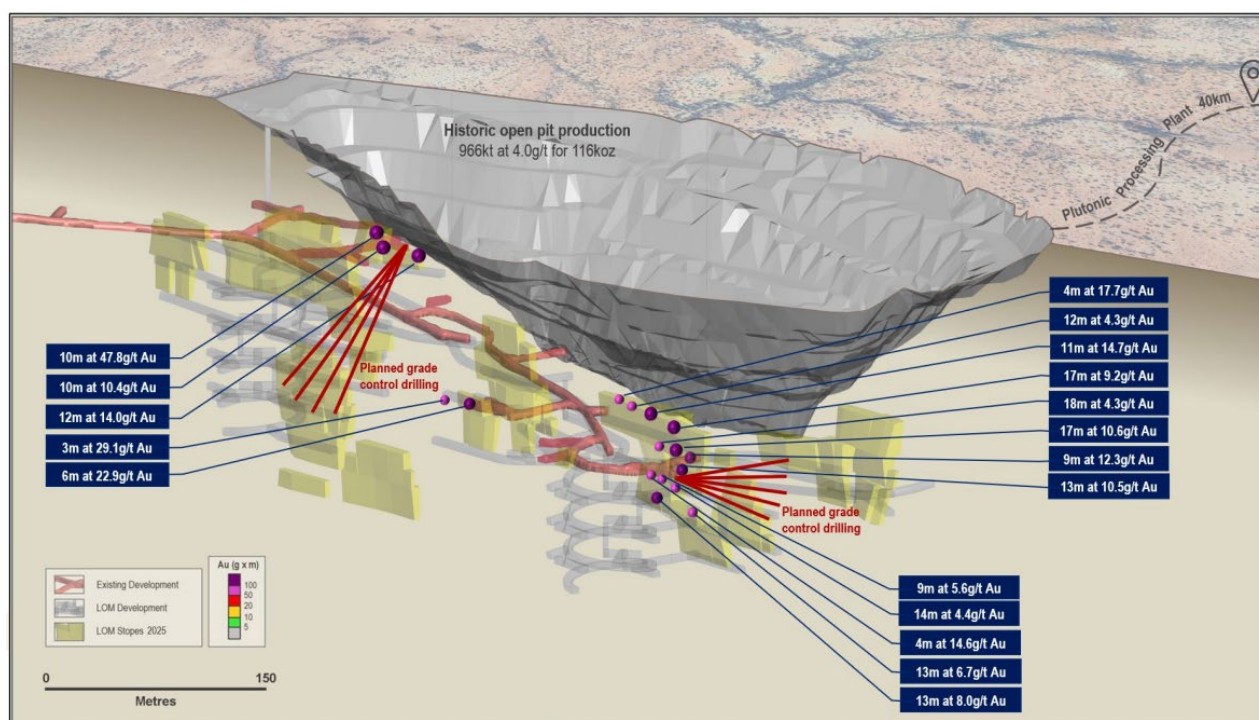
Figure 6: K2 underground mine showing development progress and recent grade control drilling results
