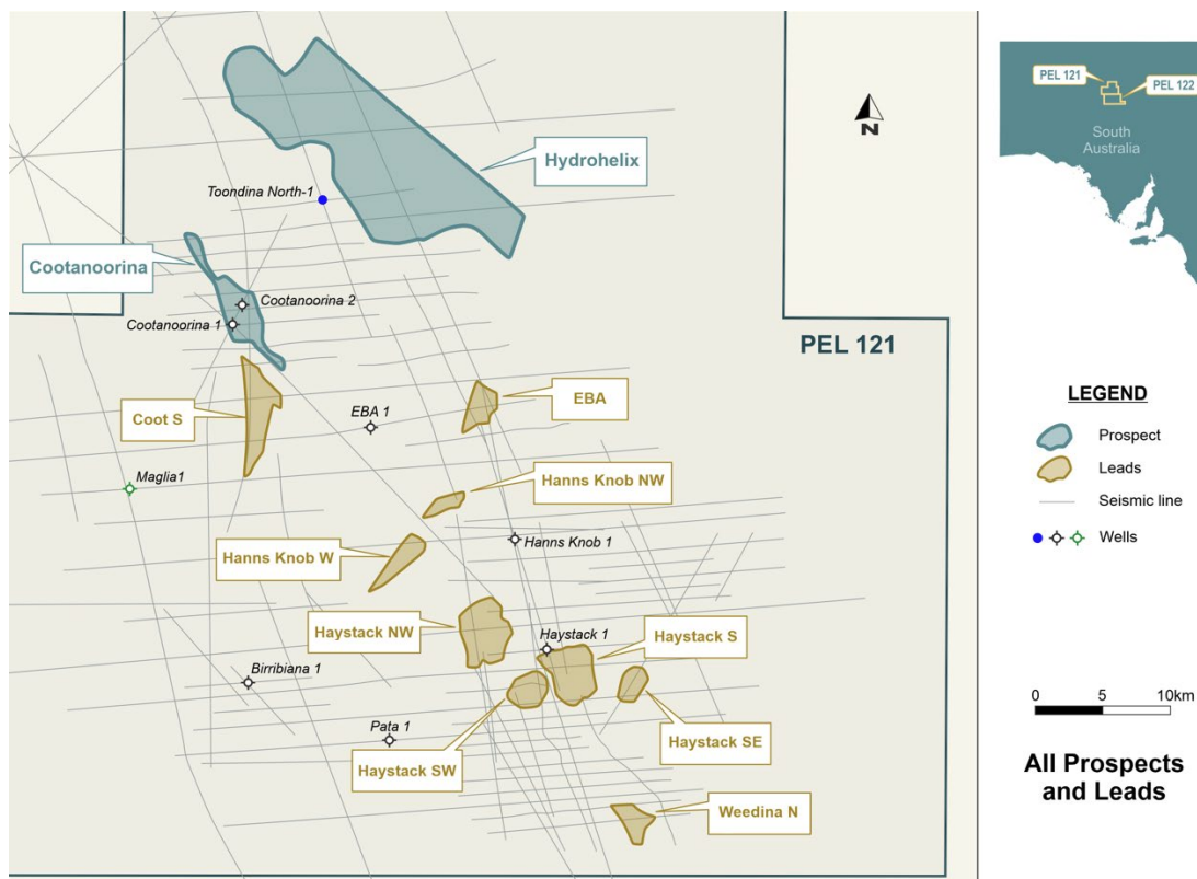
(Figure 3: Arckaringa Project Prospects and Leads)
