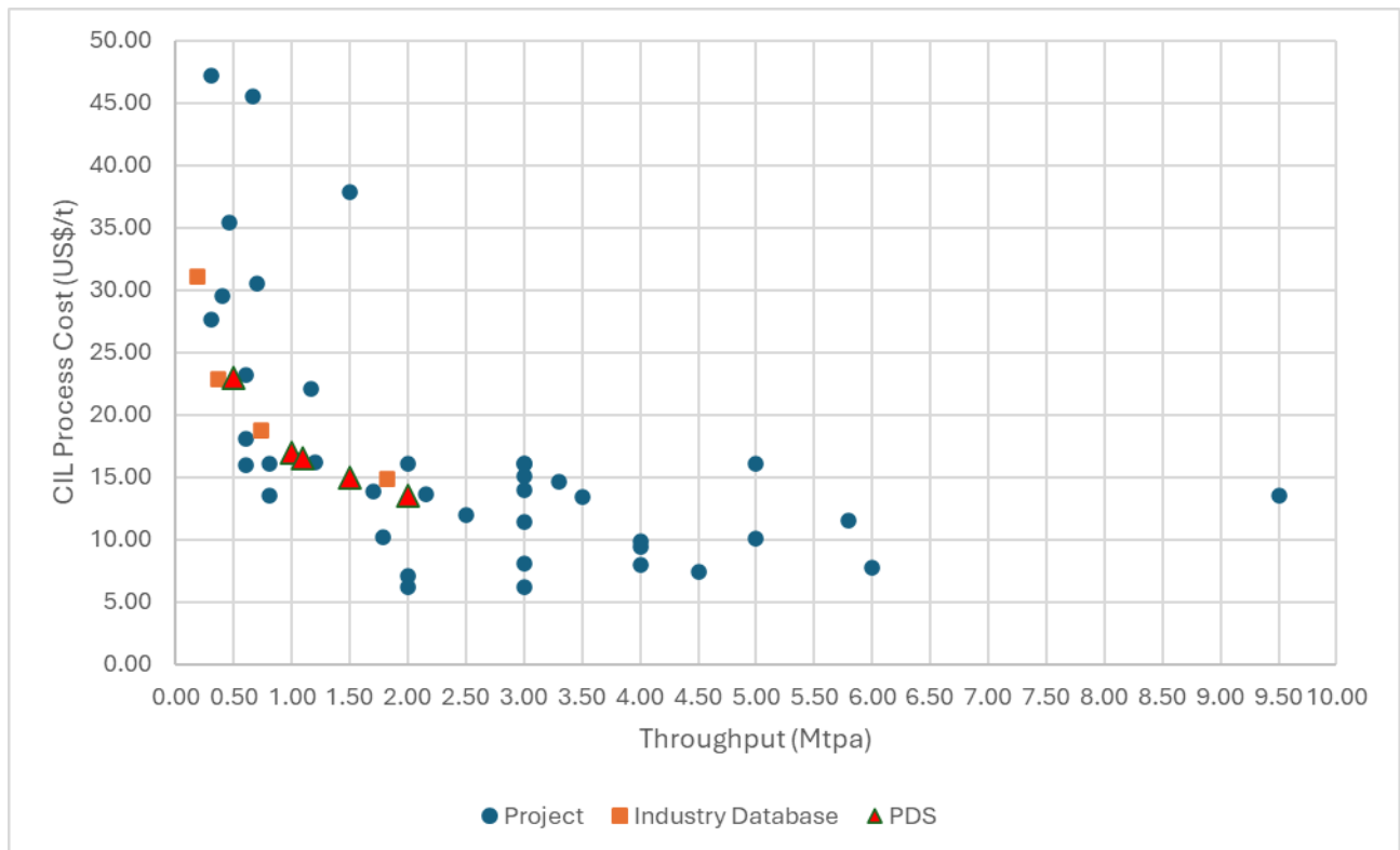
Figure 25: Benchmarking of process operating costs
