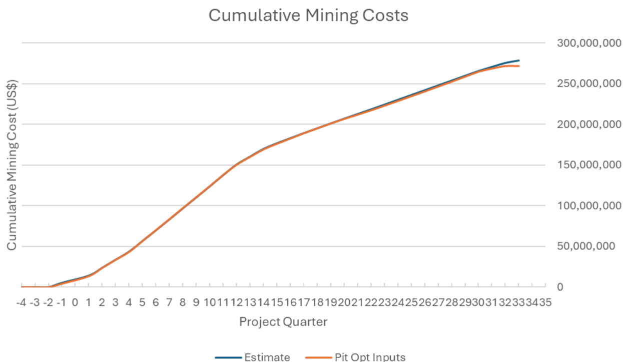
Figure 8: Check on Mining Costs for Pit Optimisation
