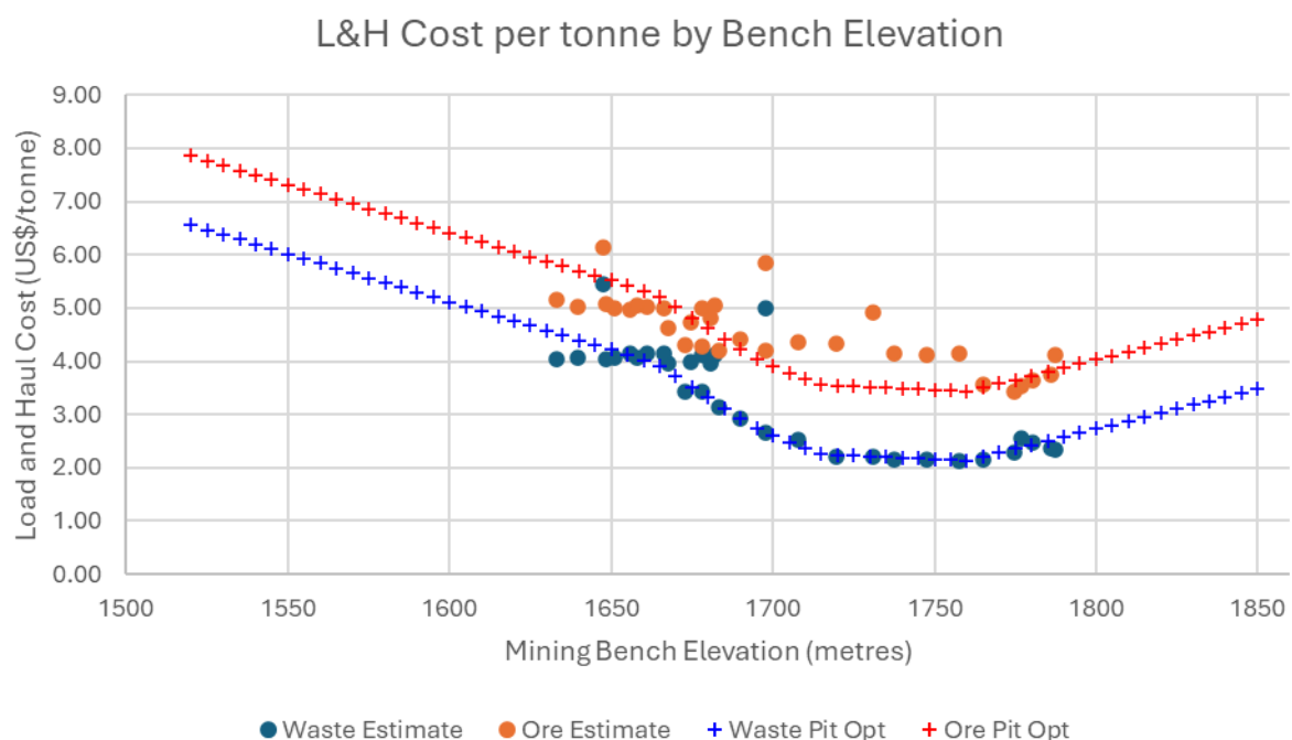
Figure 7: Mining Costs for Pit Optimisation
