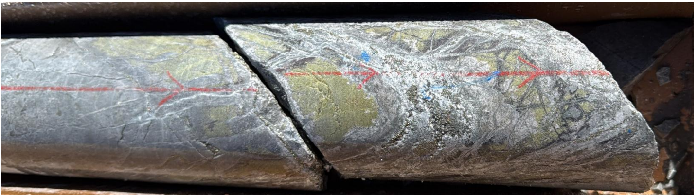
Photo 1. Epithermal mineralisation with visible chalcopyrite intersected in 25LHDD0070 from 179m (refer Table 1 and Appendix 1).
