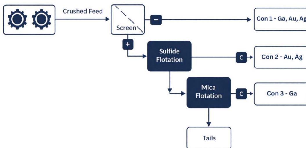
Figure 3. Phase 2 metallurgical test configuration (source: ASX announcement, 15 July 2026).
