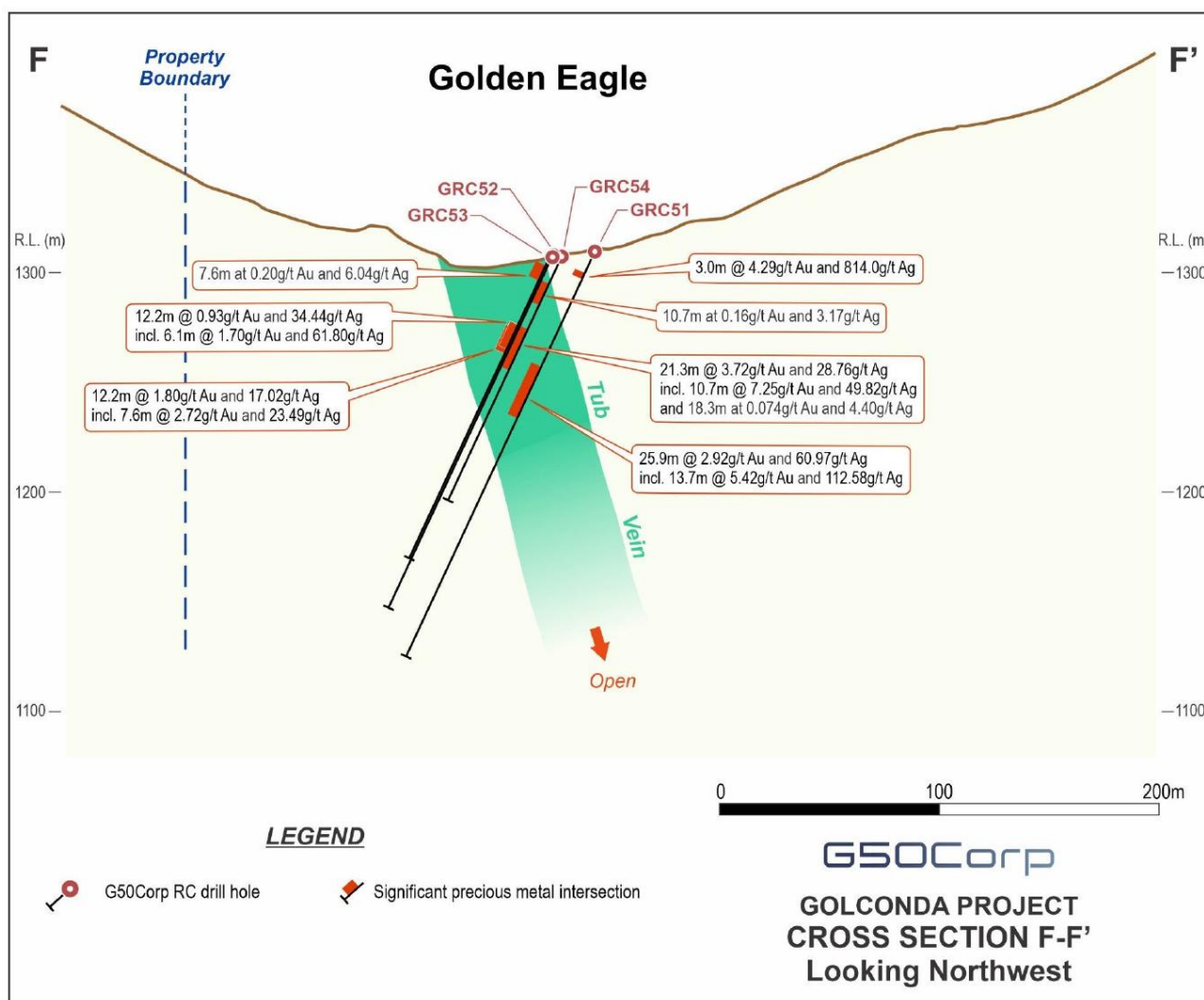
Figure 2. Cross section F to F' showing drill holes GRC51 to GRC54 at Golden Eagle, drilled over a strike length of approximately 60m (source: ASX announcement, 27 July 2026).
