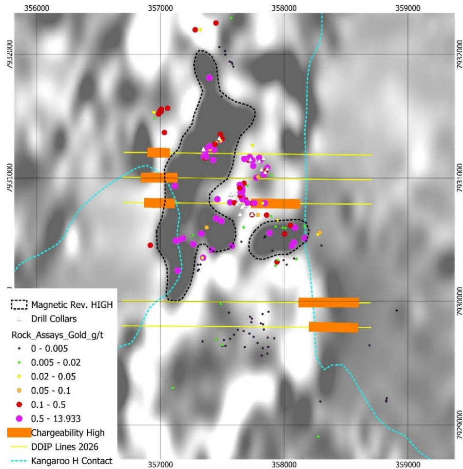
Figure 5: Airborne Magnetic Image (1VD_AGC) showing strong reverse polarised magnetic features (black dash) overlaid with the DDIP chargeability profiles anomalies (orange strips) also showing the Kangaroo Hills Formation contact (blue dash) and rock assays coloured for gold.
