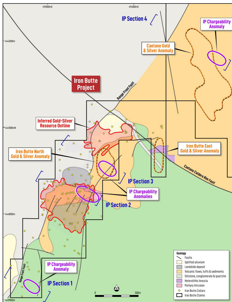
Figure 1: Geology map of Iron Butte project area showing the location of the inferred gold and silver resource and the location of four DDIP lines where the undrilled anomalies have been located.
