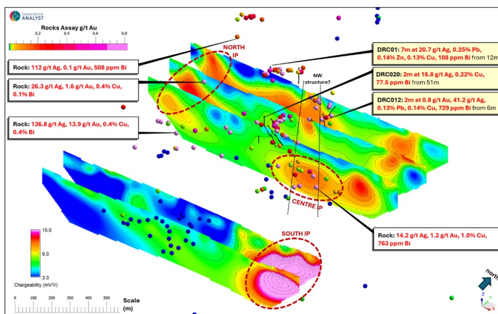
Figure 3: 3D Image of new DDIP chargeability profiles and new IP targets (red dash circles) in relation to Au in rock chips (coloured spheres), previous drilling highlights and also possible northwest structure controlling central IP anomaly.
