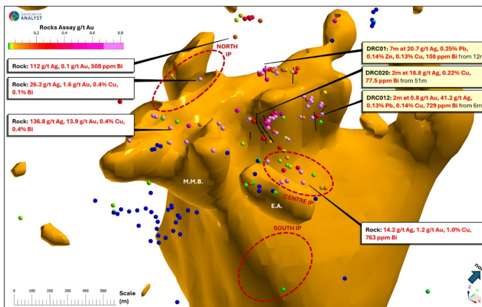
Figure 4: 3D Image of Airborne Magnetic Inversion of strongly reverse polarised body (orange) highlighting the main magnetic body (M.M.B.) and eastern apophysis (E.A.) in relation to Au in rock chips (coloured spheres), previous shallow drilling highlights and newly identified IP chargeability anomalies (red dash).
