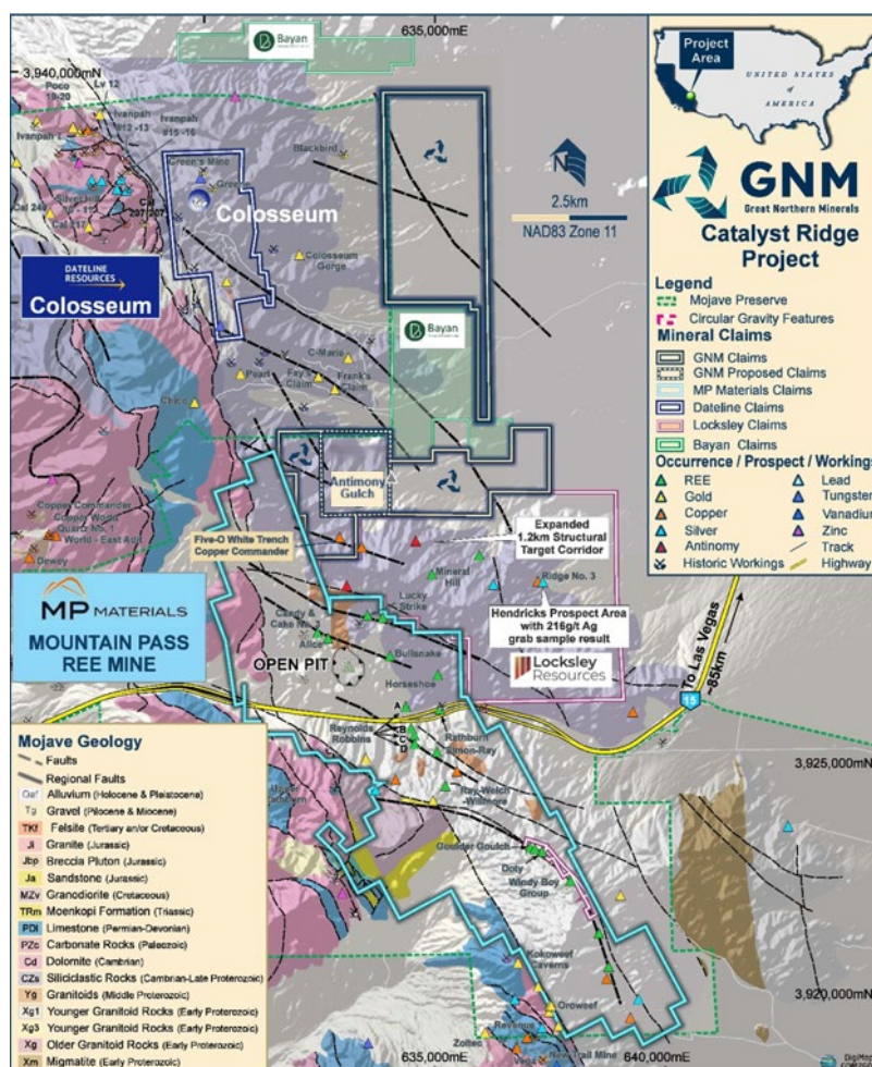
Figure 6: Interpreted bedrock geology map from the US Geological Survey 1 showing the location of GNM's existing and proposed new claims in relation to associated nearby mineral occurrences and other companies in the area.
