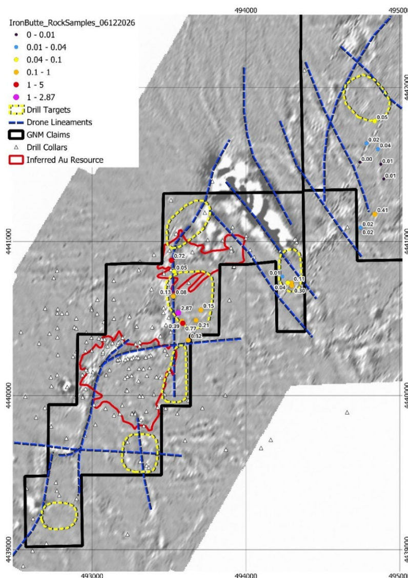
Figure 2: UAV Magnetic image (2VD TMIRTP) of the Iron Butte project area showing the location of the inferred gold resource, preliminary structural interpretation and location of drill targets (yellow dash).
