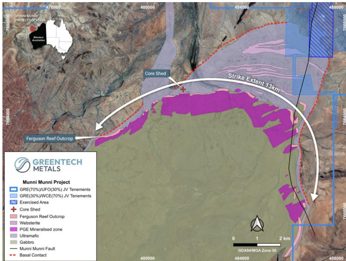
Figure 4: Map of northern extent of Munni Munni intrusion highlighting basal zone target.
