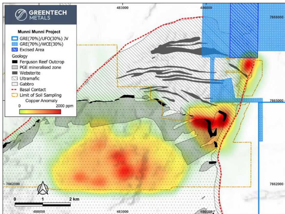
Figure 3: Soil copper geochemistry over the Munni Munni intrusion, showing the base of the ultramafic sequence (dashed red outline) – a high-priority target zone to be investigated by the FLEM survey and drill program
