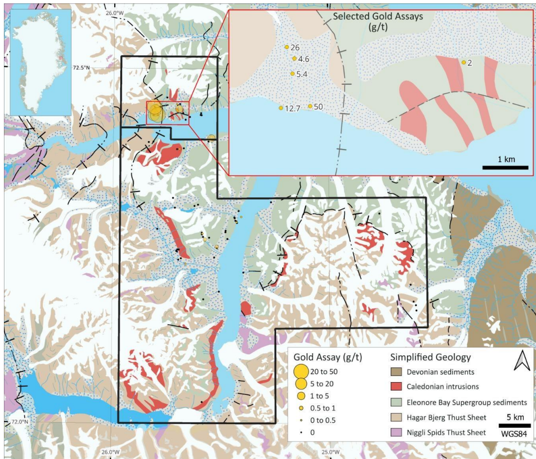
Figure 5: Simplified geological map with historical Nordmine grab sample gold results. The inset map shows the location of selected historical high-grade grab samples from Table 2. All results are available in Appendix 1 of the announcement dated 4 August 2026.
