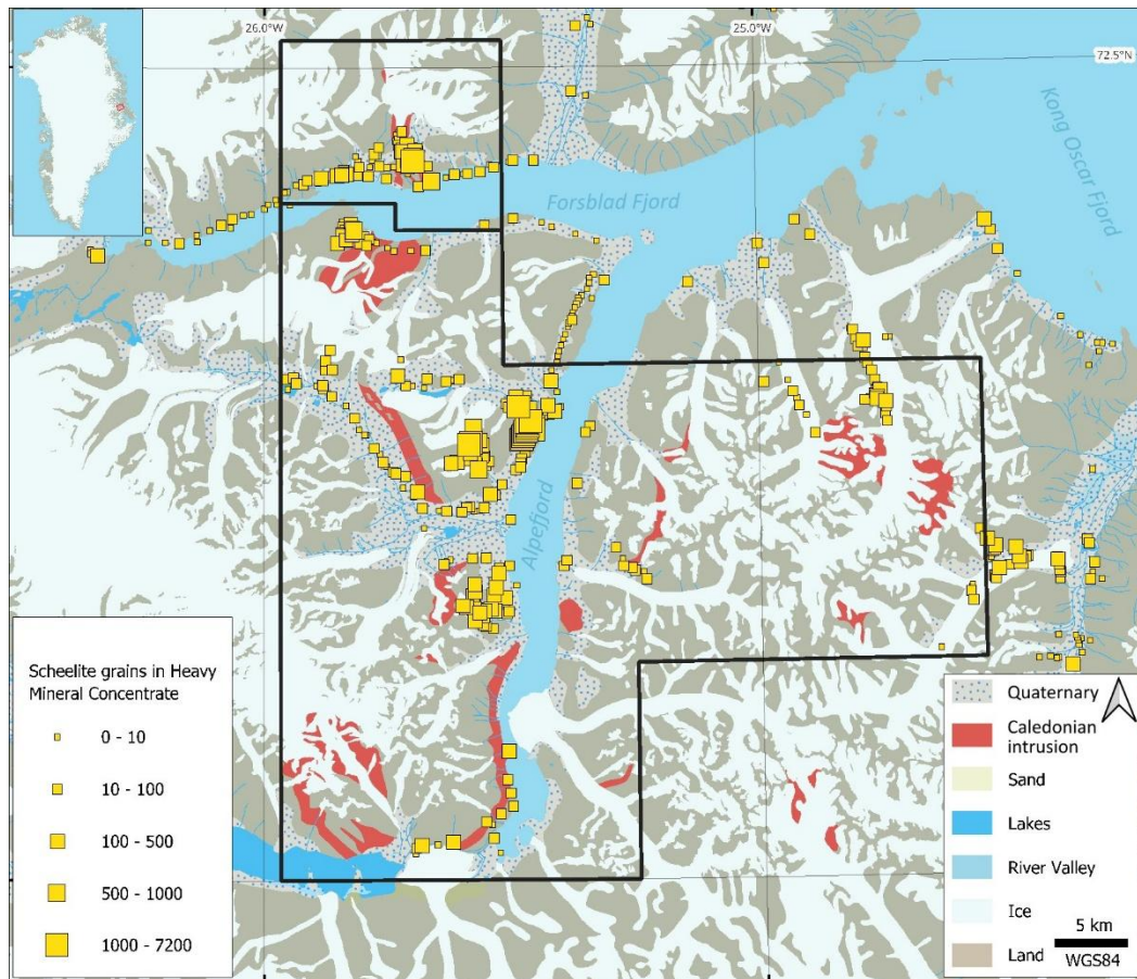
Figure 6: Scheelite grain count in historical panned heavy mineral concentrate samples.
