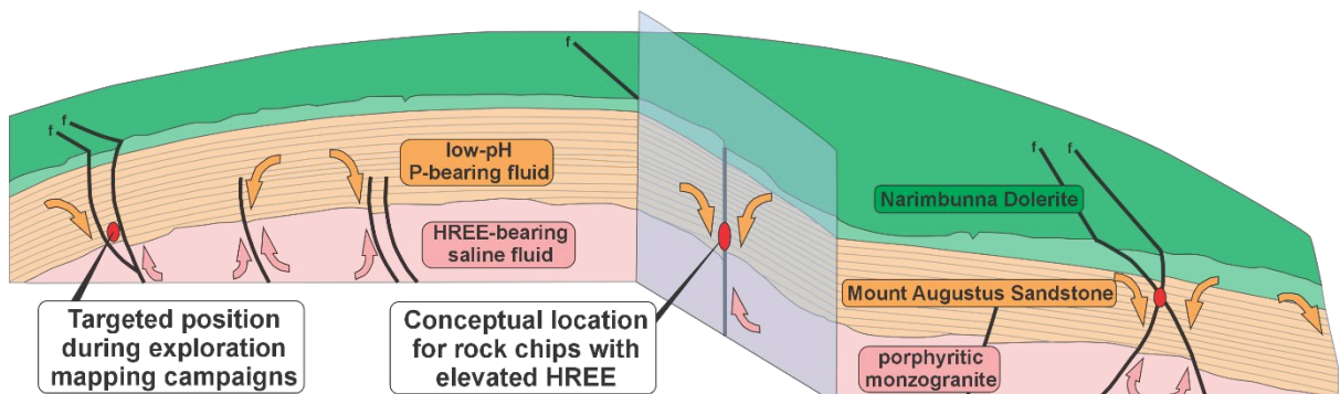
Figure 6 Schematic section illustrating the conceptual model of HREO and uranium mineralisation; (modified from Nazari-Dehkordi, 2018).
