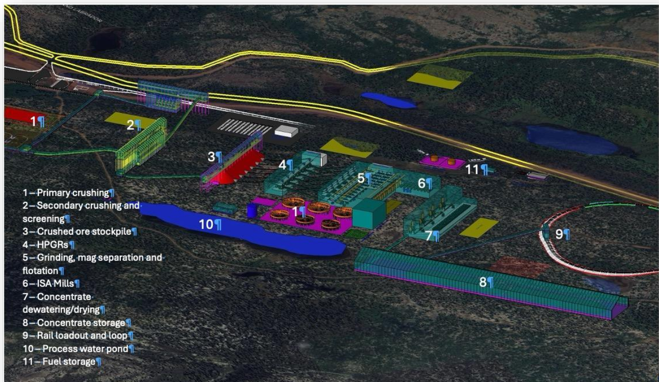
Figure 3. 3D model of processing plant showing crushed ore stockpile, grinding and separation, drying and process water pond plus concentrate storage before railing
