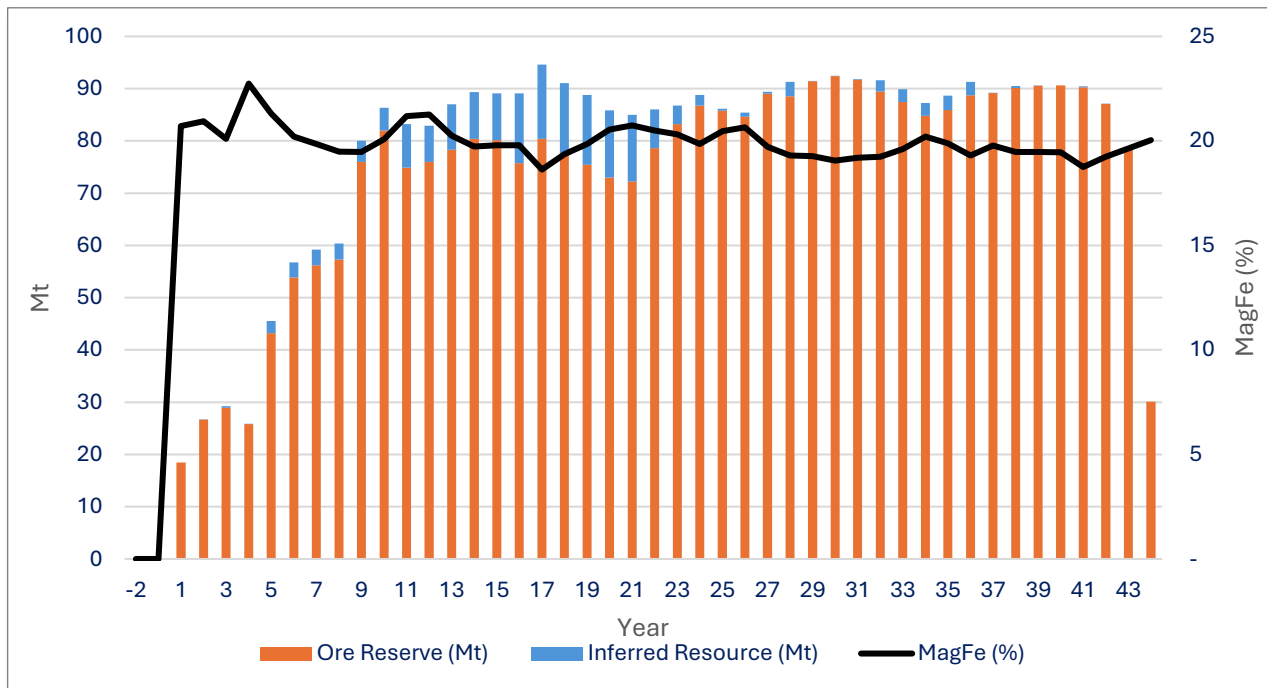
Figure 2. Process Feed Quantities and Grade by classification
