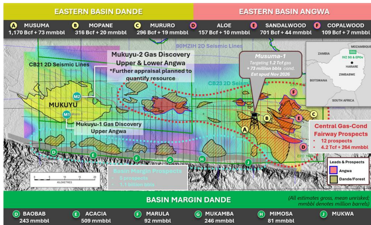
Figure 3 – Cabora Bassa portfolio showing Mukuyu Gas Field, Musuma-1 target, and leads and prospects in the project area.
