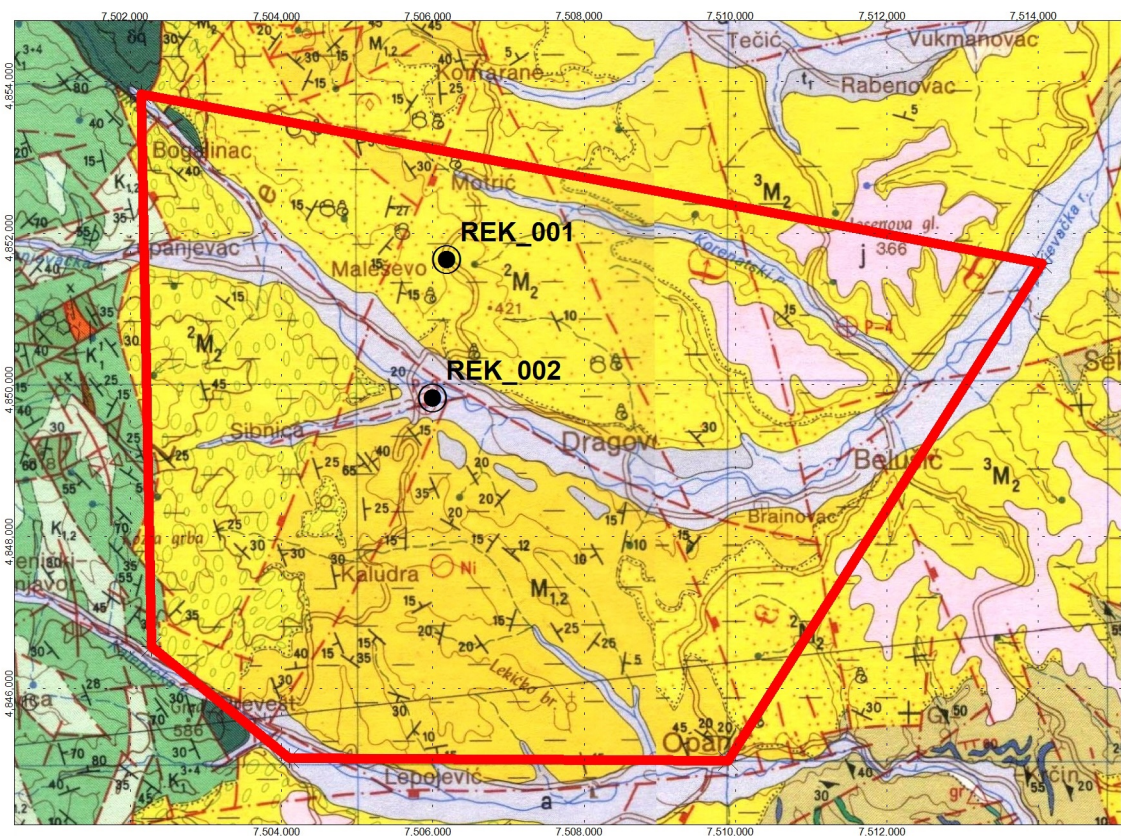
Figure 2 – Position of Drill Holes
