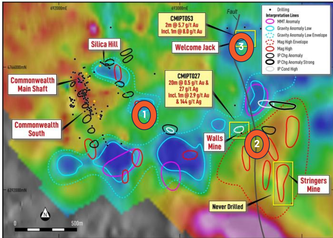
Figure 2: Integrated geophysical targeting across the Commonwealth-Silica Hill Project, highlighting a prominent magnetic intrusive complex southeast of Silica Hill coincident with gravity, IP and MobileMT anomalies. The geophysical response is interpreted to represent a potential buried intrusive system and provides a compelling target for porphyry-style mineralisation analogous to the intrusive-related system interpreted at Silica Hill. The Welcome Jack prospect, Walls and Stringers all occur along the same fault line within the Welcome Jack Corridor as indicated. Previously reported by Kuniko in ASX announcement dated 21 August 2026.
