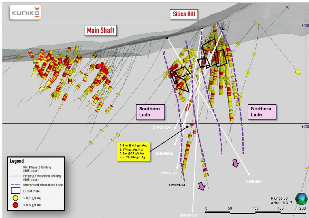
Figure 1: Oblique 3D view of the Silica Hill-Commonwealth Main Shaft mineralised system, showing Kuniko Phase 2 drilling (white lines), historical drilling, interpreted Northern and Southern Lodes, gold assay distribution and historical DHEM conductor plates (black outlines). Previous DHEM surveys successfully identified conductive targets associated with sulphide mineralisation at Silica Hill coupled with compelling drill hole intercepts. The deeper Phase 2 drill holes provide an opportunity to extend DHEM investigations below the existing mineralised system and identify potential off-hole conductors for follow-up drilling. Highlighted is the high-grade intersection in CMKNI004 of 0.5 m at 27 g/t Au and 20,603 g/t Ag, demonstrating the potential for high-grade precious metal mineralisation associated with massive sulphide veins at Silica Hill.
