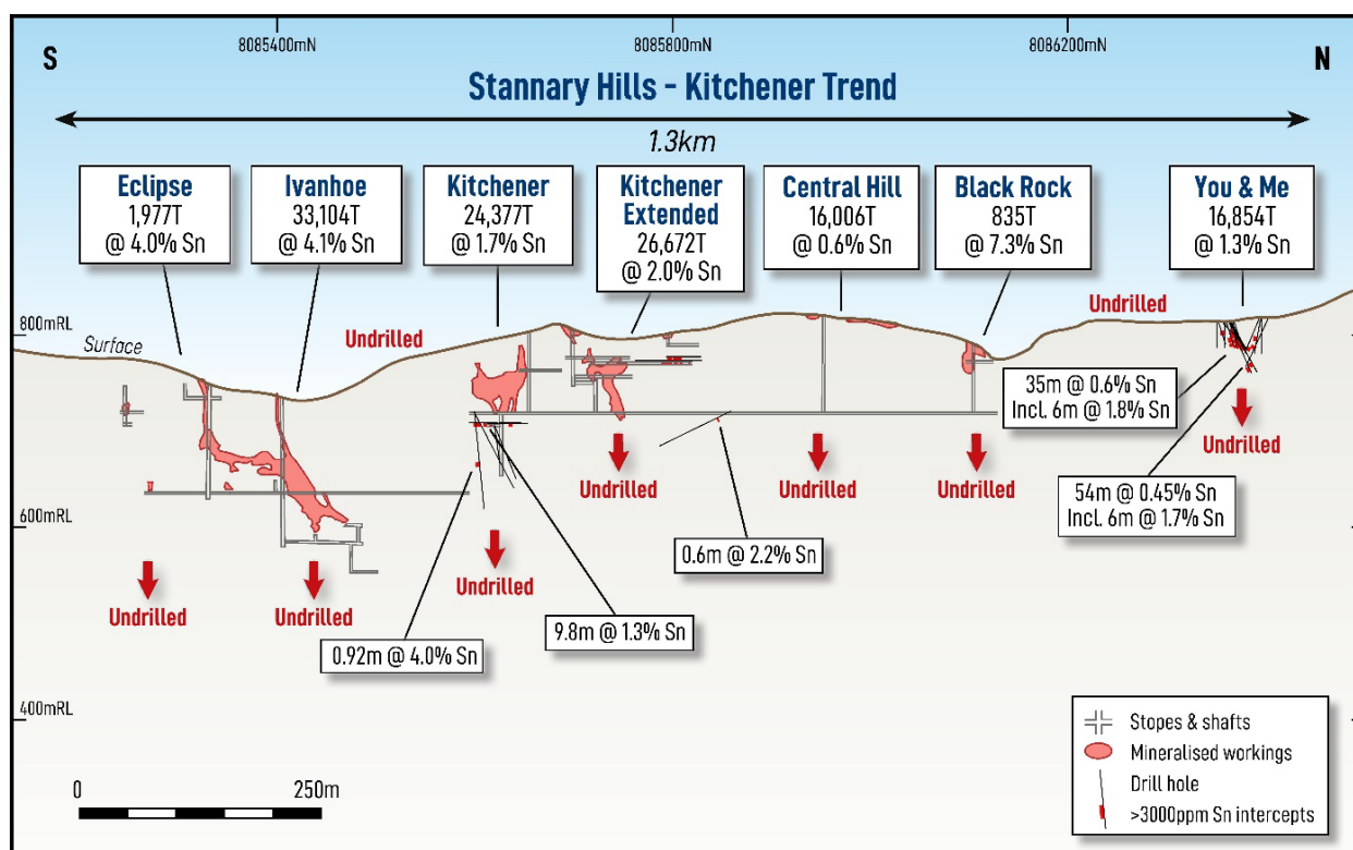
Figure 5. Long section showing a group of seven high-grade historical tin mines over 1.3km of strike along the Kitchener Trend. Note that only very limited drilling has been completed both between historical mines and at depth – providing substantial opportunity for discovery of significant tin mineralisation.
