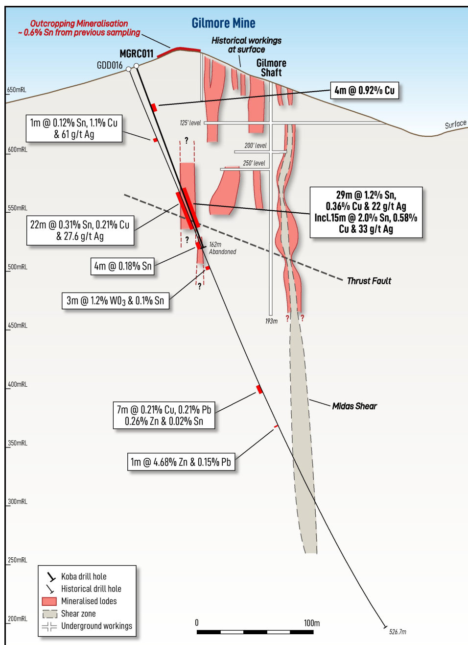
Figure 3. Cross-section through the Company's recent drill hole MGRC011 at the Gilmore Tin Mine. The location of the section is shown in Figure 2.
