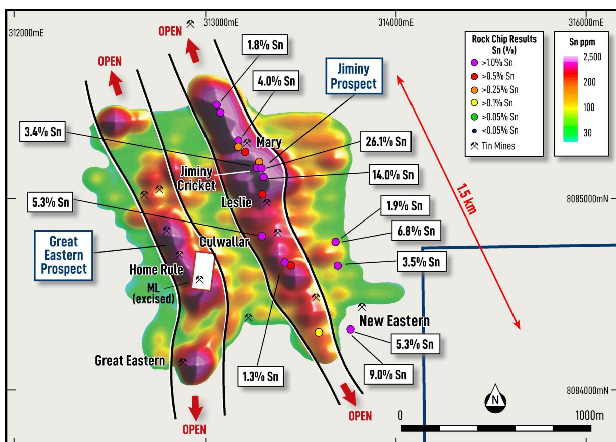
Figure 6. Assay results from recent rock chip sampling plotted on an image of tin-in-soil geochemistry at the Jiminy Prospect and adjacent Great Eastern Prospect areas, within the Stannary Hills Tin-Tungsten Project.
