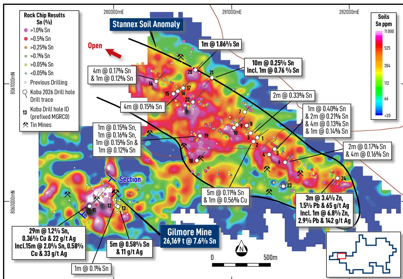
Figure 2. Drill hole location plan showing significant intersections from Koba's maiden RC drilling at the Gilmore Tin Mine and Stannex Prospect, Mt Garnet Tin-Tungsten Project.
