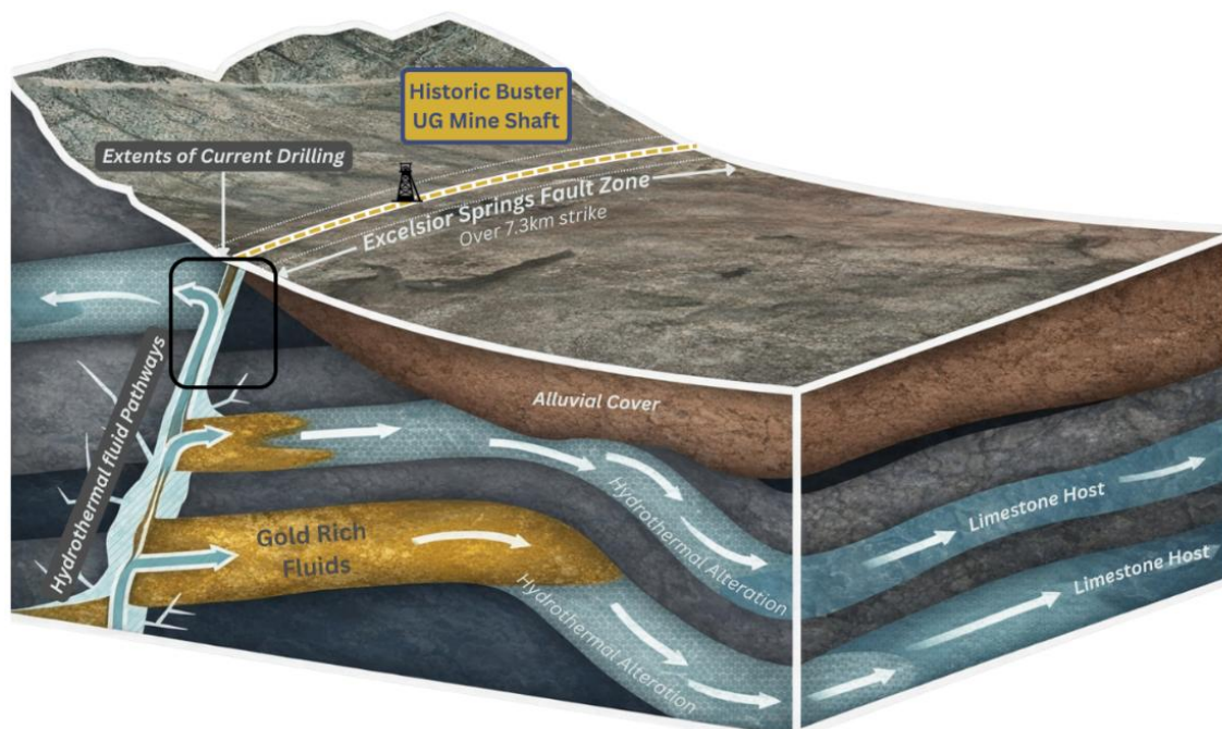
Figure 5: Schematic of Carlin-Type Gold Deposit model at Buster Trend Excelsior Springs
