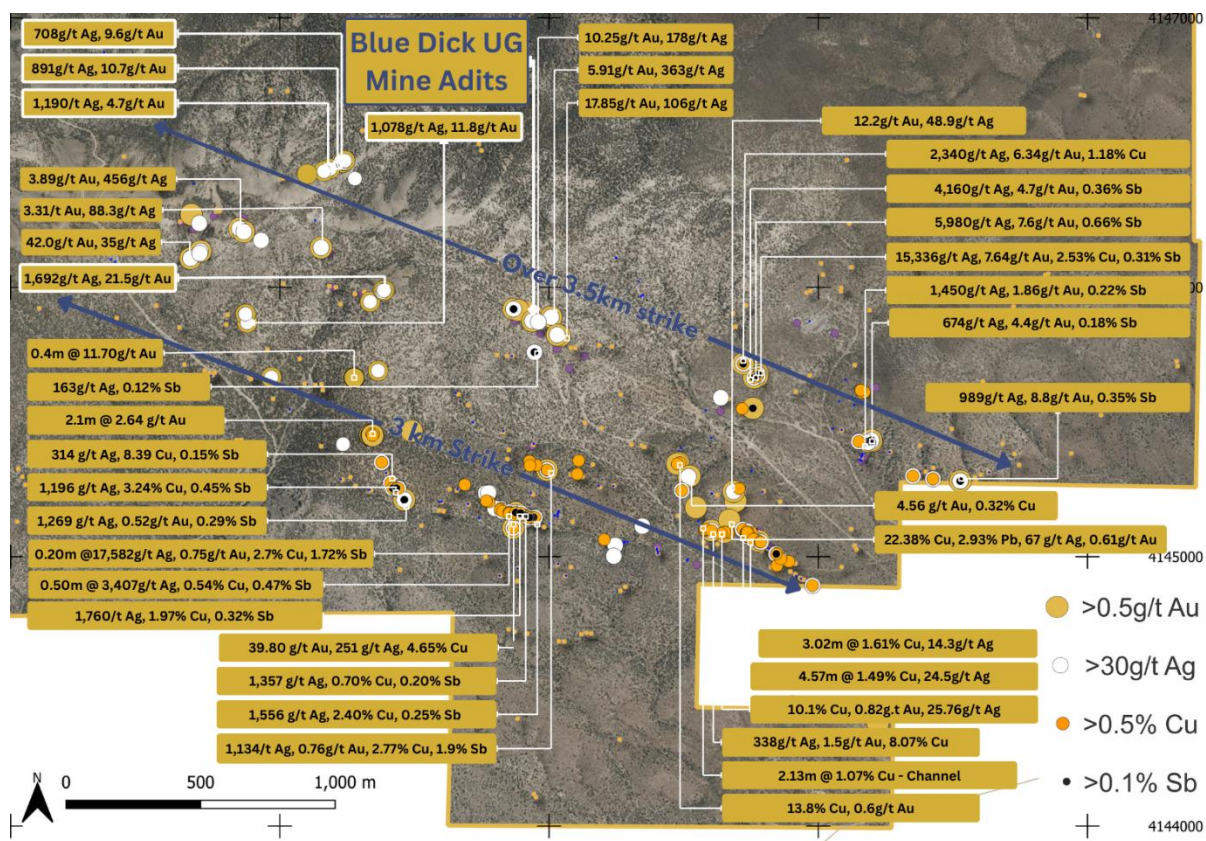
Figure 4: Surface sampling results from across the Blue Dick Prospect Area, with latest results outlines shown in white
