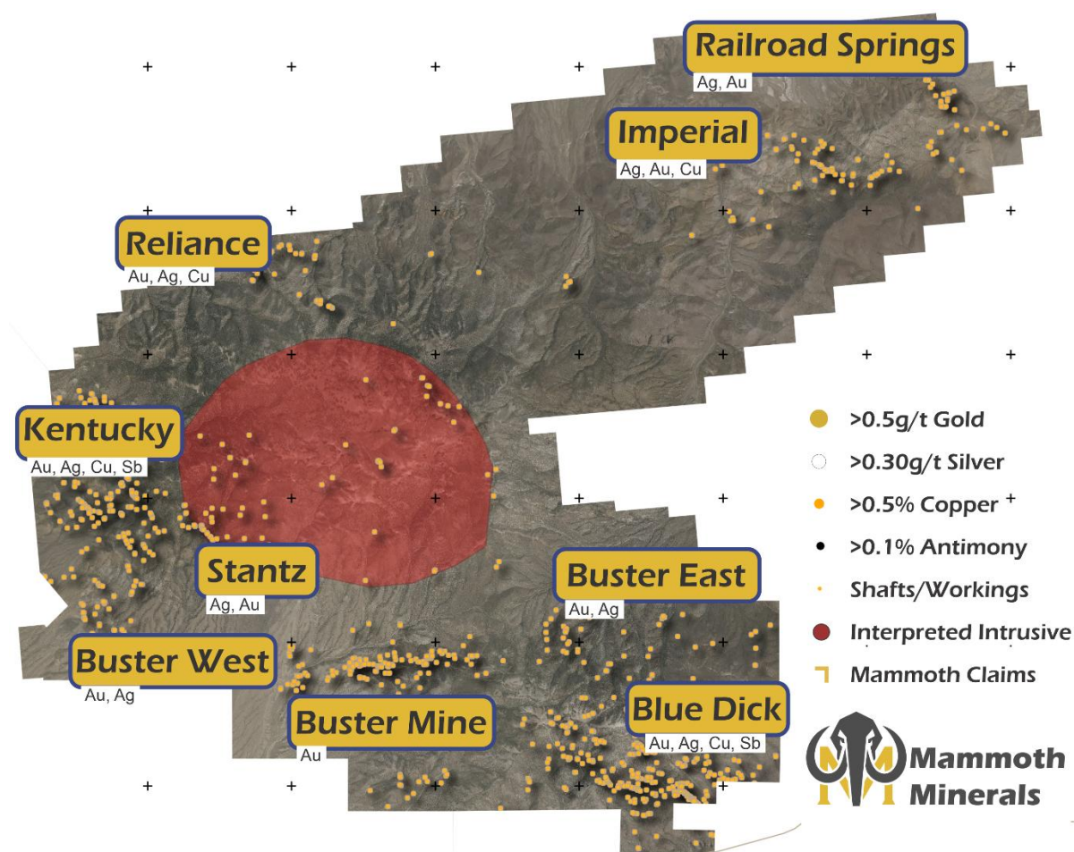
Figure 3: Excelsior Springs Mineral Claim targets overview
