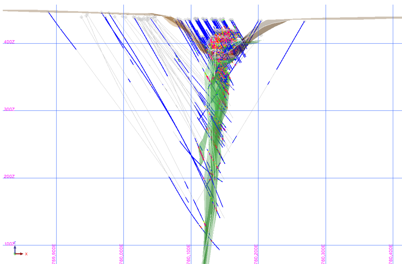
Figure 10: Cross section of the mineralisation wireframes used to estimate the Blue Vein Mineral Resource.
