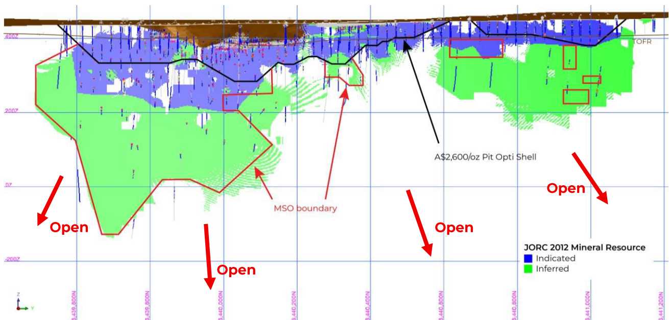
Figure 12: Long section showing Blue Vein Mineral Resource classification.
