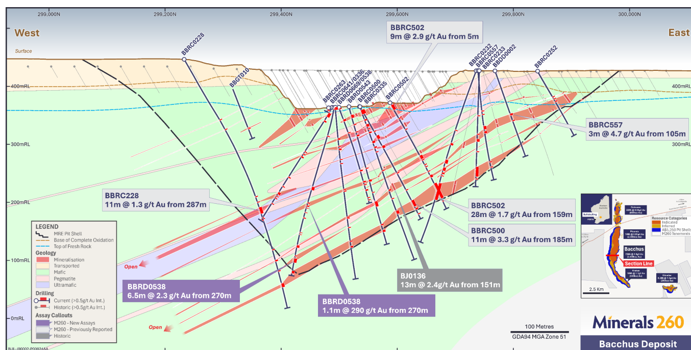
Figure 8: Section 6566330N showing mineralisation in BBRD0538 infilling Bacchus MRE pit shell (new results in purple boxes)
