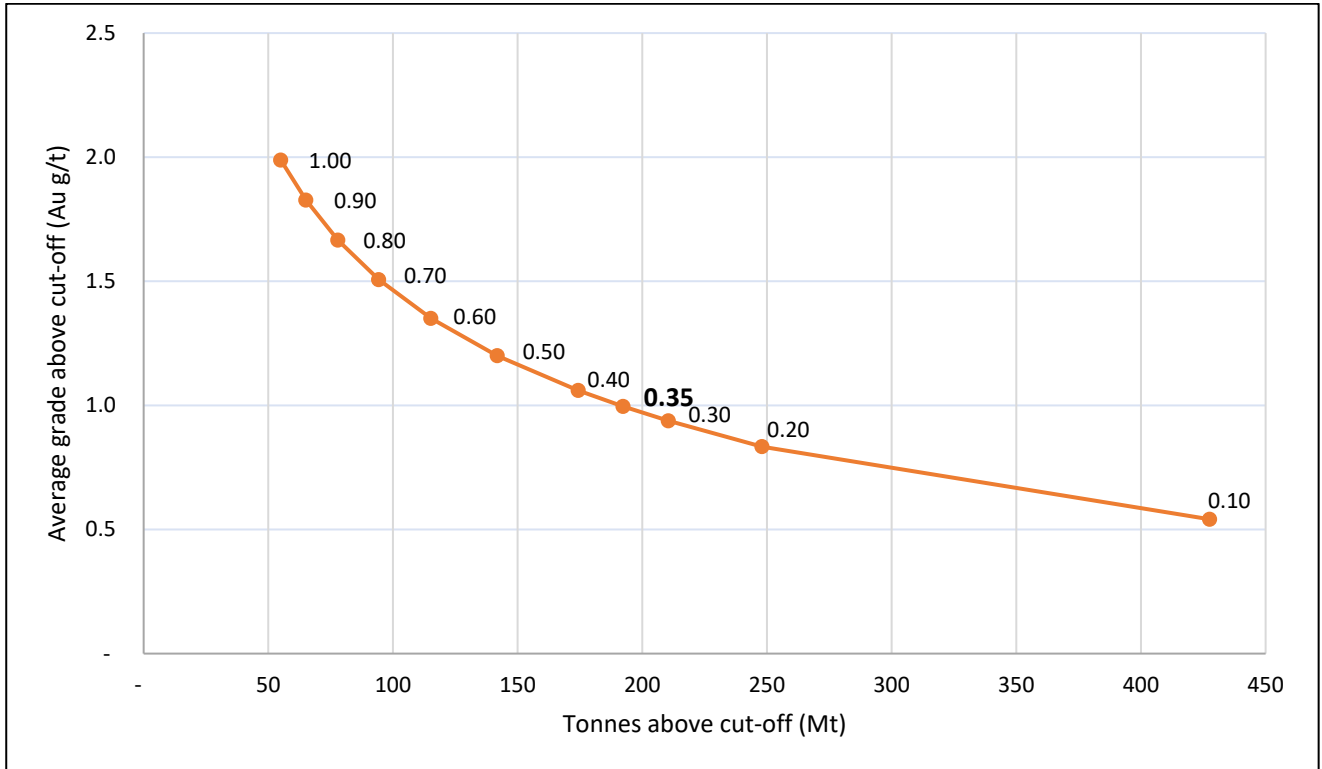
Figure 3. Grade-tonnage Curve for Mineralisation within the A$5,250/oz Au Pit Shell
