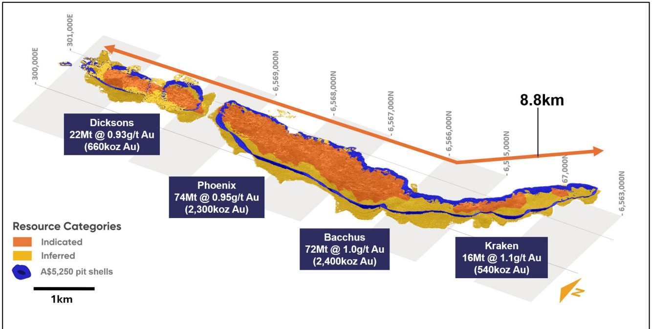
Figure 6. Bullabulling MRE 3D Model Showing Resource Classification within the A$5,250/oz Au Pit Shell (looking north-east)
