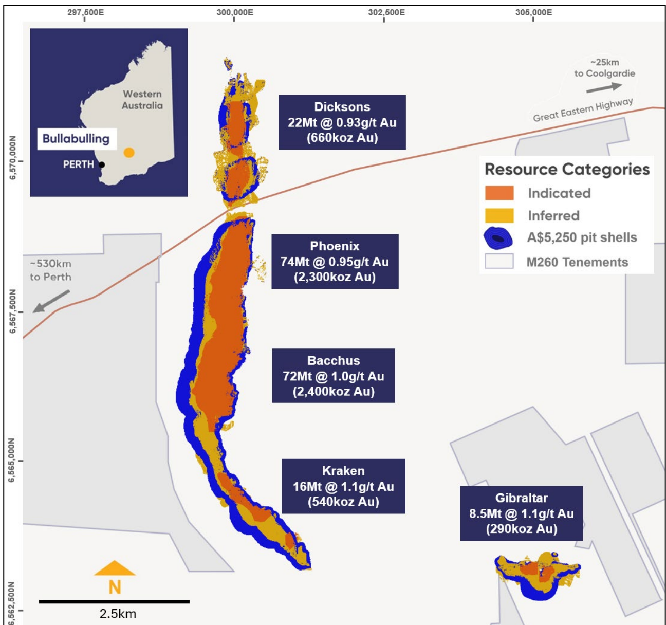
Figure 5. Bullabulling MRE Plan Showing Resource Classification within the A$5,250/oz Au Pit Shell
