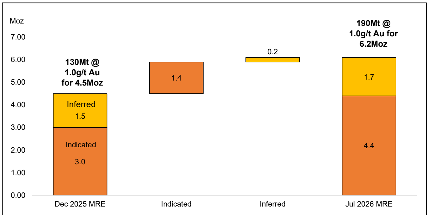
Figure 2. Changes in MRE (Moz Au) by Classification Category
