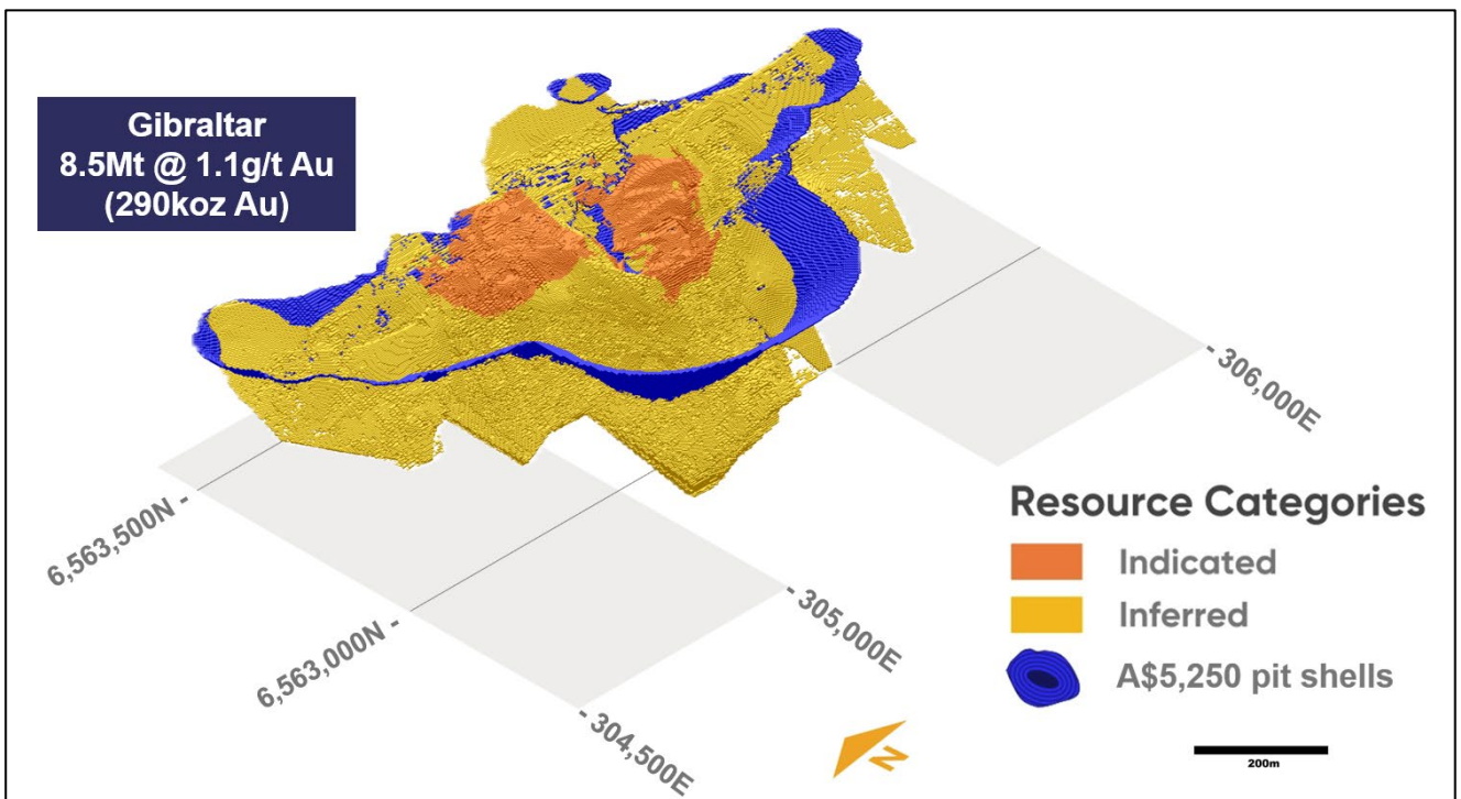
Figure 7. Gibraltar MRE 3D Model Showing Resource Classification within the A$5,250/Oz Au Pit Shell (looking north-east)
