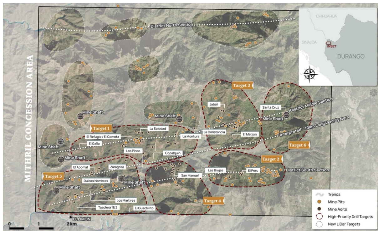
Figure 2 LiDAR identified historic workings across the 70km² district. Current drilling locations at Target 1 west and Target 5 (El Apomal), and recent drilling at Zaragosa mine in Target 1 south, high priority drill target area of La Constancia-El Jabali (Target 3). Several new areas highlighted across the district for follow-up work including recently sampled Target 6
