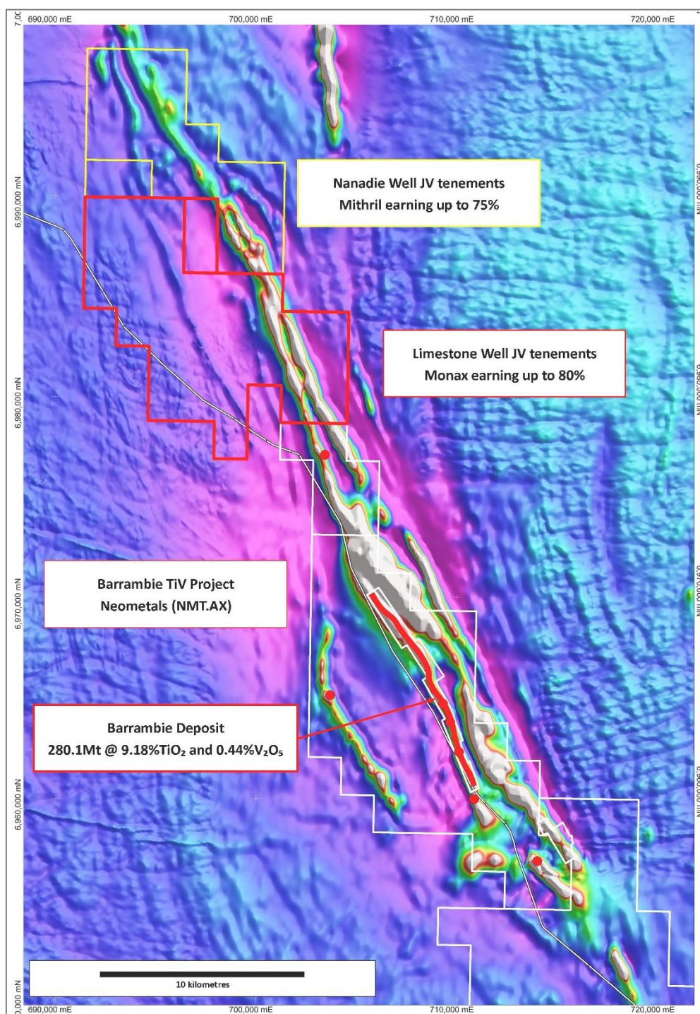
Figure 2: Regional magnetic image showing location of the Barrambie Deposit and the Limestone Well JV tenements (red outline) and Mithril's Nanadie Well JV tenements (yellow outline) where it is earning up to 75%.
