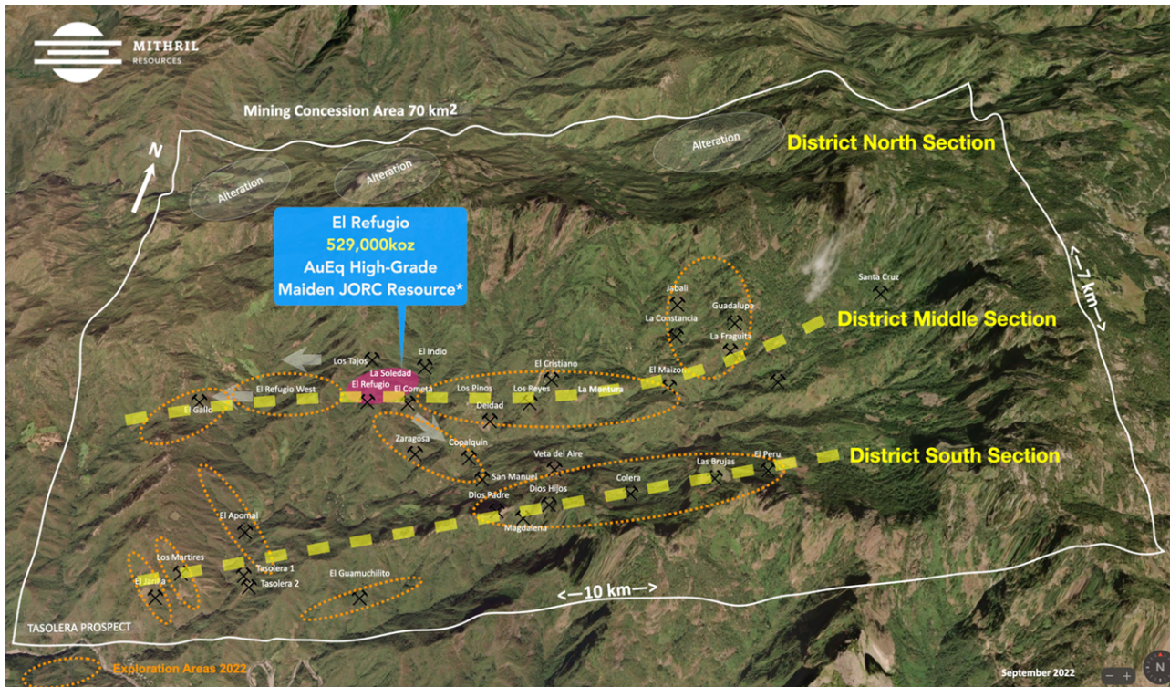
Figure 2 – Satellite image of the Copalquin Mining District 70km² concession area showing the two main lines of historic workings, areas of exploration work and the location of the maiden JORC MRE at El Refugio. The long sections indicated on the map are shown in the figures below.
