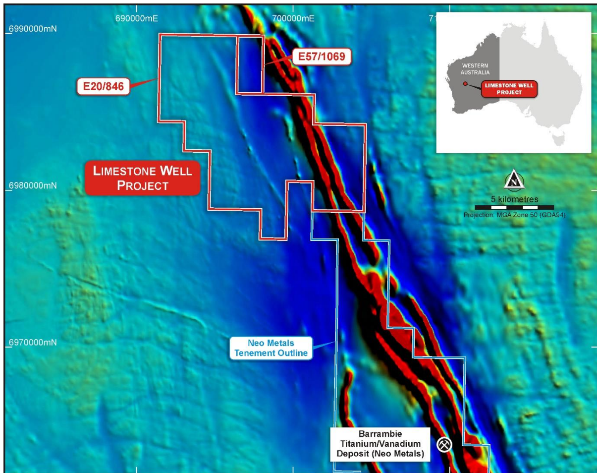
Figure 2: Magnetic image showing the Limestone Well Project and prospective rock units
