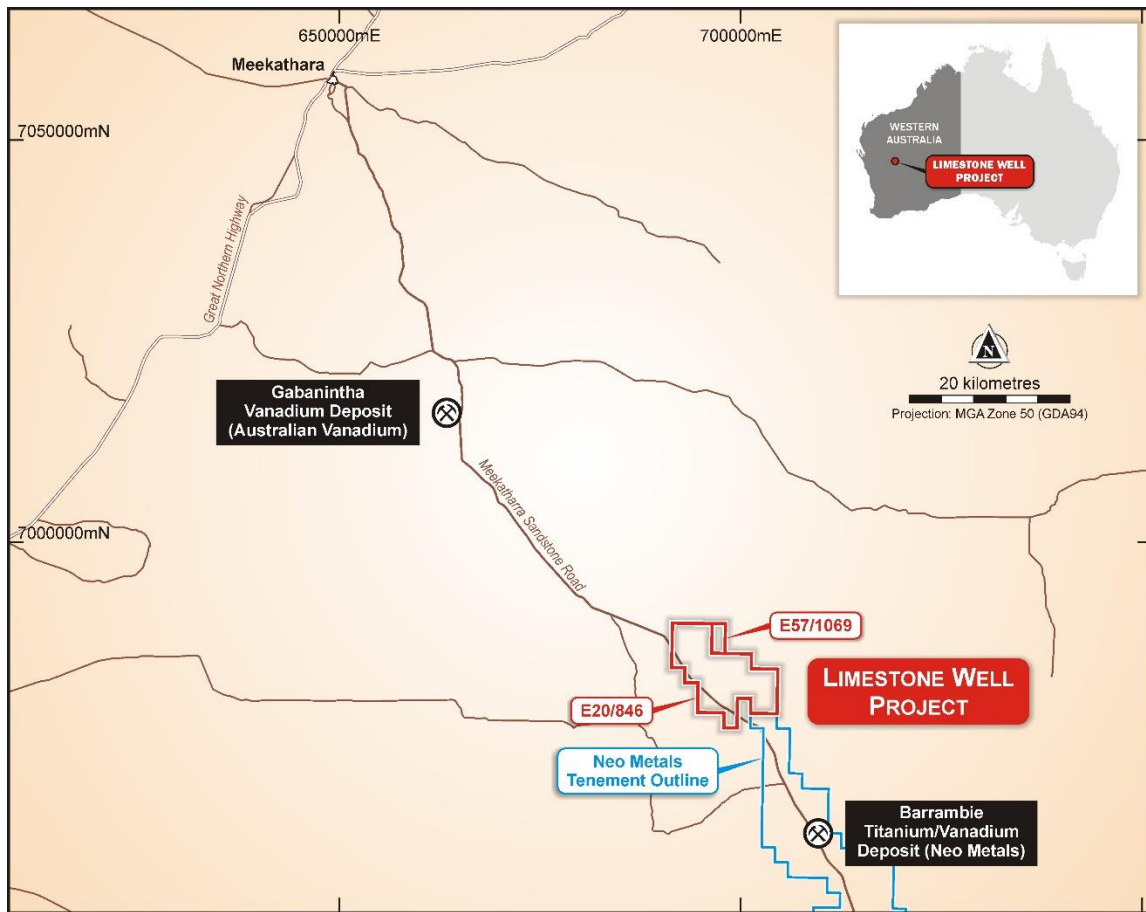
Figure 1: Limestone Well project location plan
