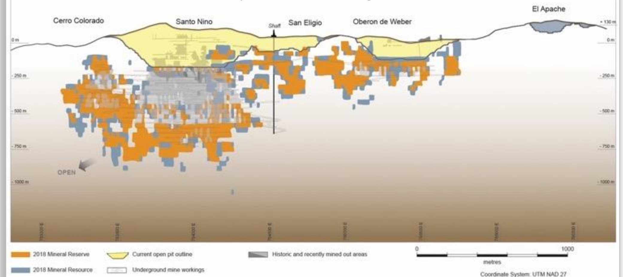
Nearby Los Pinos Mine Log Section
