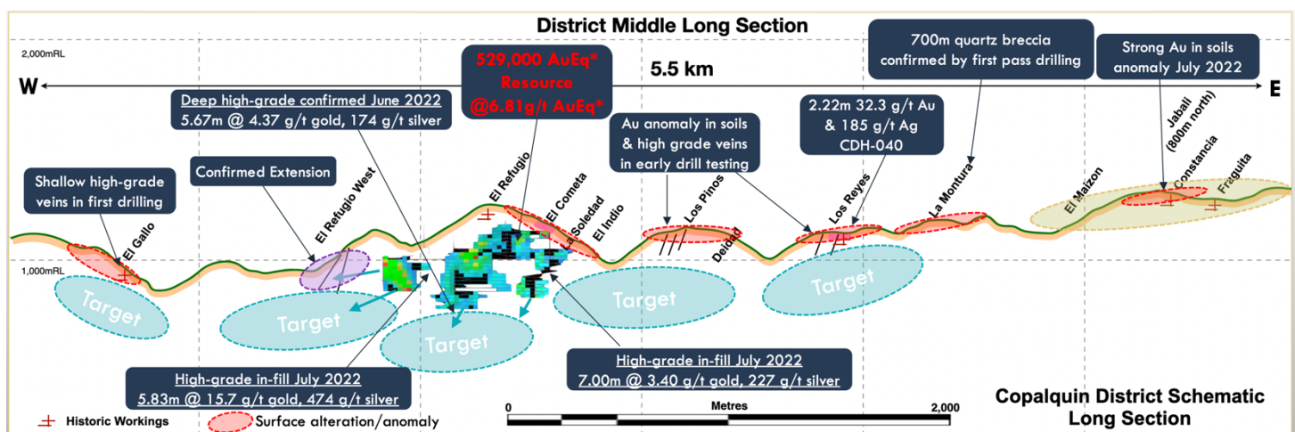
Figure 11 – Schematic long section of the Copalquin District Middle Section which includes the maiden JORC resource at El Refugio/La Soledad.
