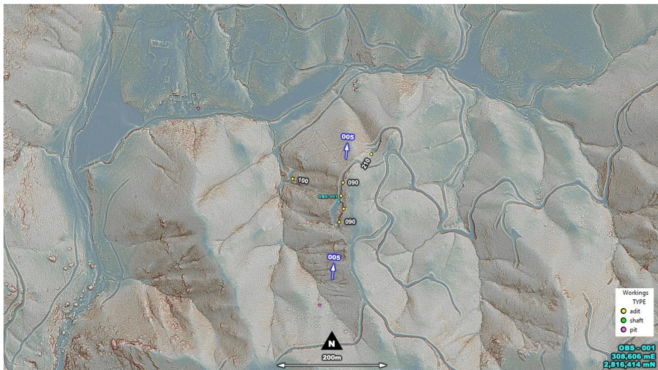
Figure 11 OBS-001: Multiple adits aligning a 005 azimuth are driven East into the ridgeline. The 210 trending adit just to the NE sits ~20 m lower elevation to the adit chain that appears driven towards the same structure. Adit azimuth labels in white text.
