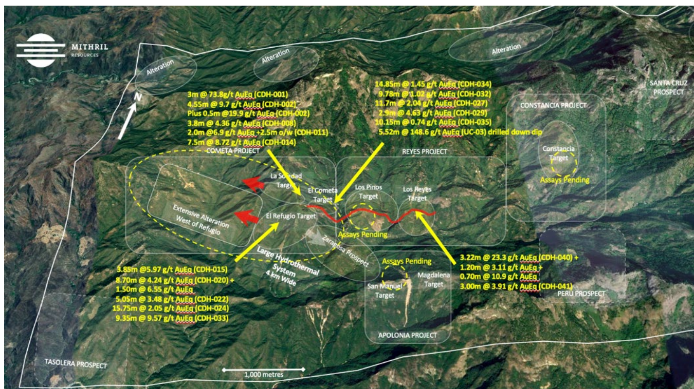
Figure 8: Projects and Prospects within the Copalquin District with drilling highlights to-date from the maiden drill program.
