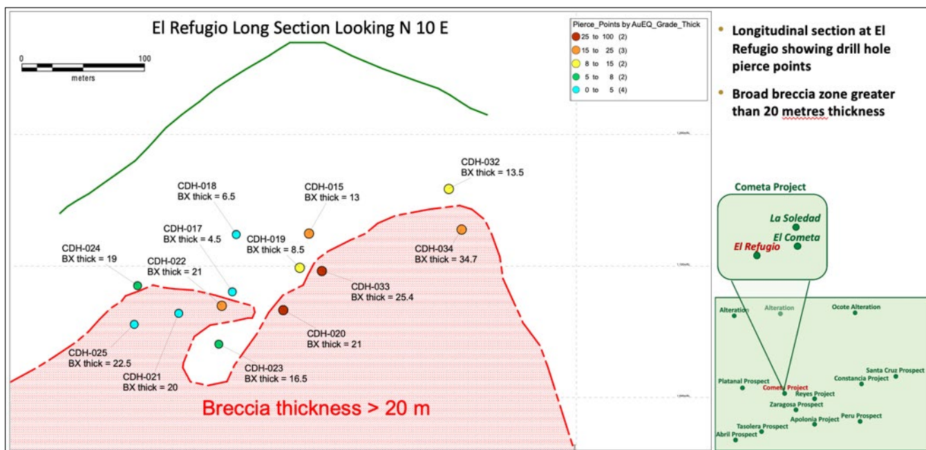
Figure 5: El Refugio long sections showing drill hole pierce points and the breccia zone where it exceeds 20 metres in width.
