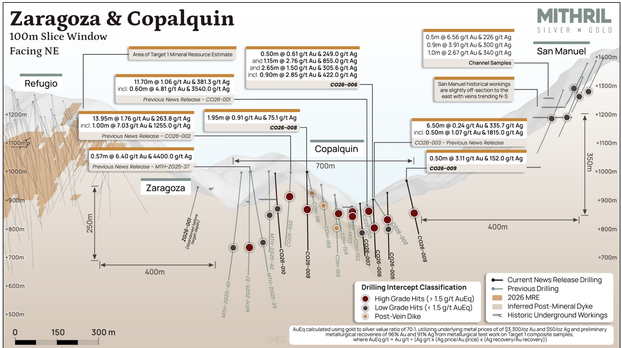
Figure 2: Long section view of the Copalquin-Zaragoza vein looking perpendicular to vein to the northeast
