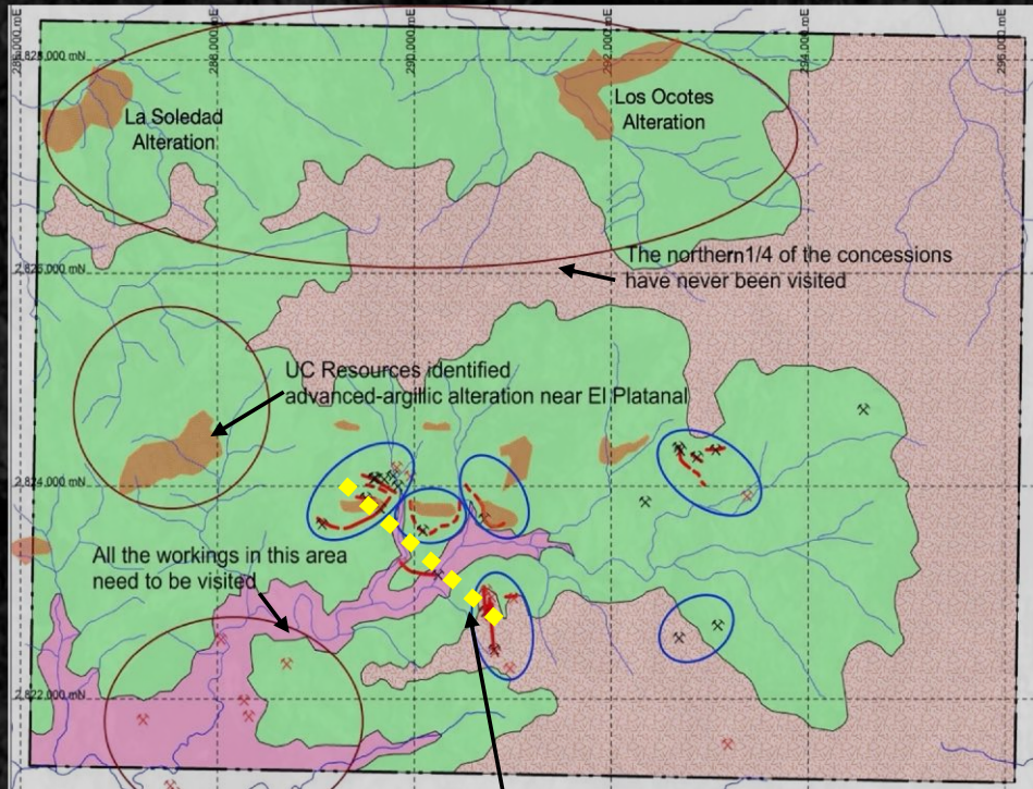
Geologic Model Section
