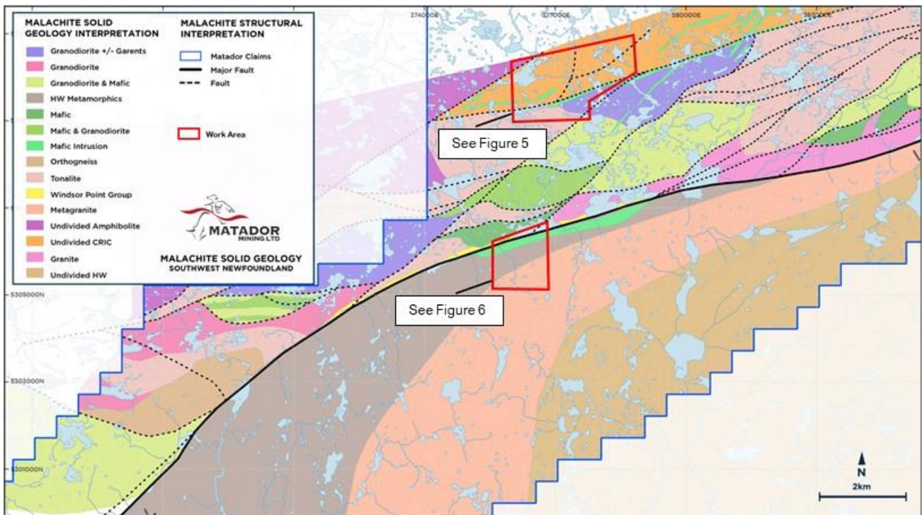
Figure 4: Updated solid geology interpretation based on integration of 2022 mapping constraints with Matador's high resolution 2021 heli-magnetic dataset
