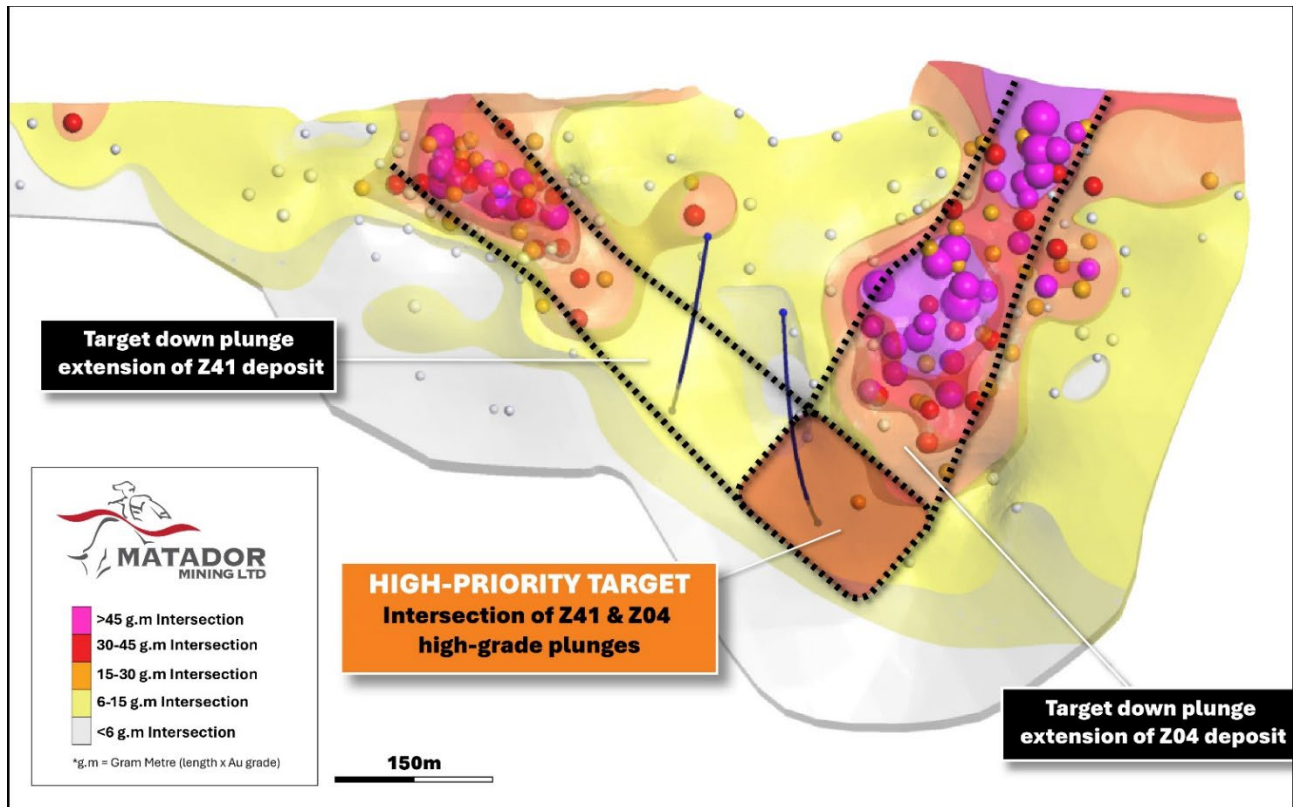
FIGURE 3: LONG SECTION OF THE Z04 & Z41 DEPOSITS SHOWING DOWN-PLUNGE OPPORTUNITIES
